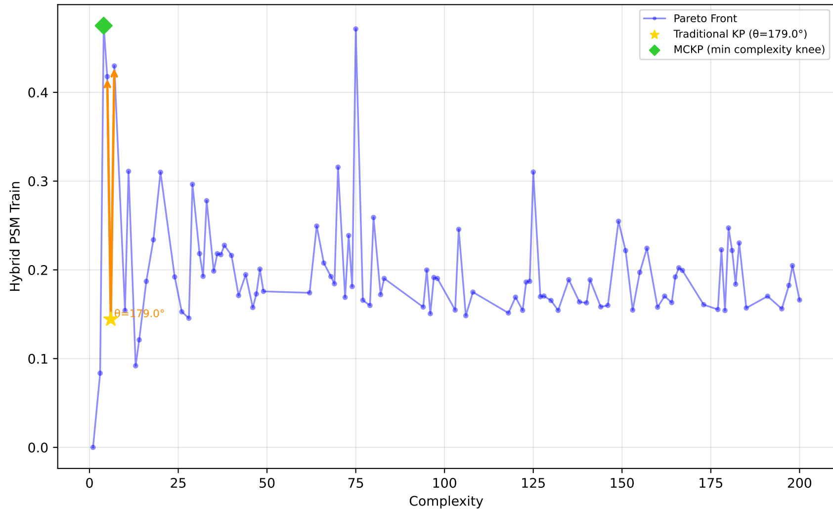
542_pollution - Run 15 - MVP - Hybrid PSM Train \lambda_1=1.00, \lambda_2=0.10, \lambda_3=0.00 | Difficulty: 0.42 | Method: mckp
