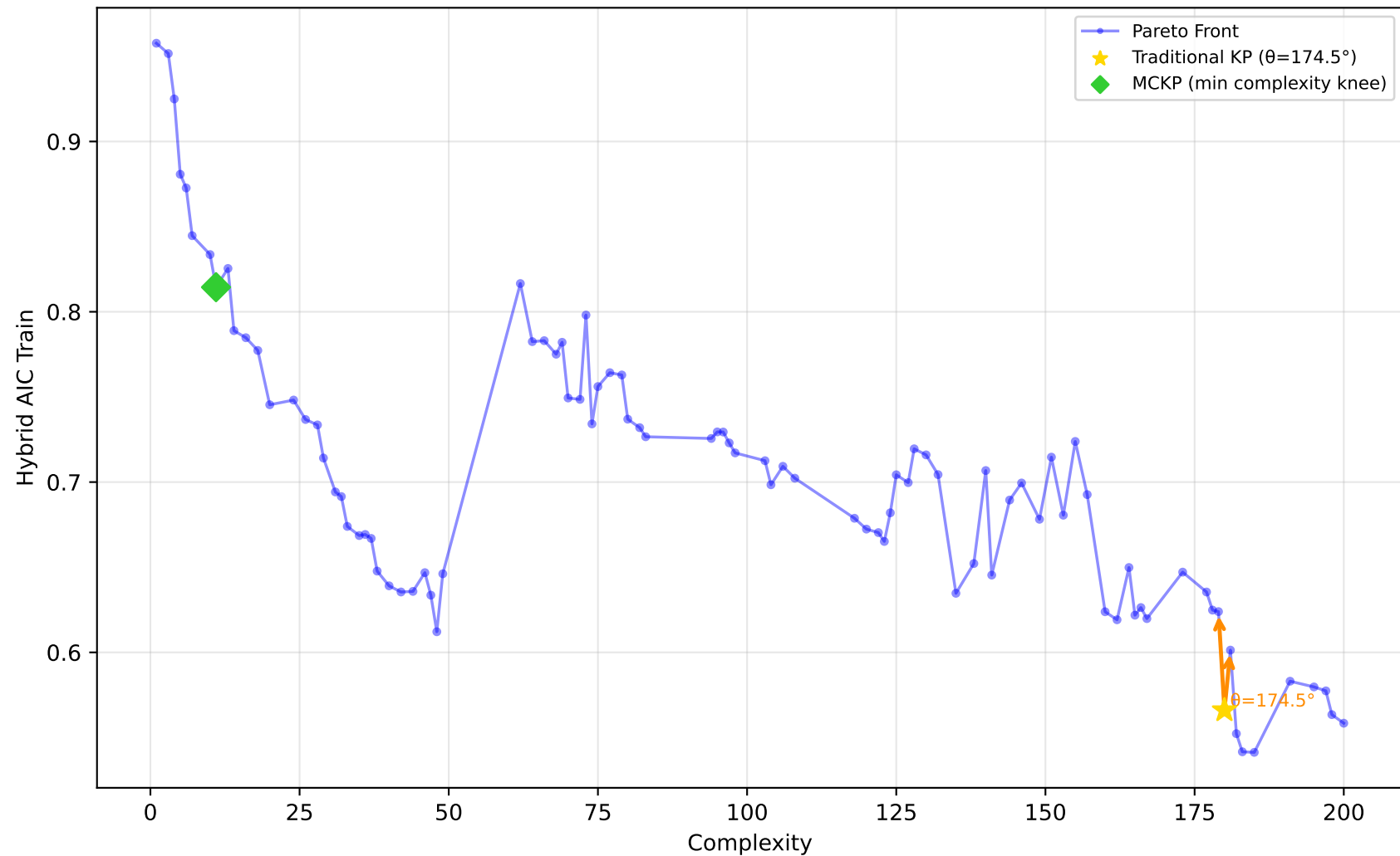
542_pollution - Run 15 - SVP - Hybrid AIC Train \lambda_1=0.00, \lambda_2=0.00, \lambda_3=0.20 | Difficulty: 0.42 | Method: mckp
