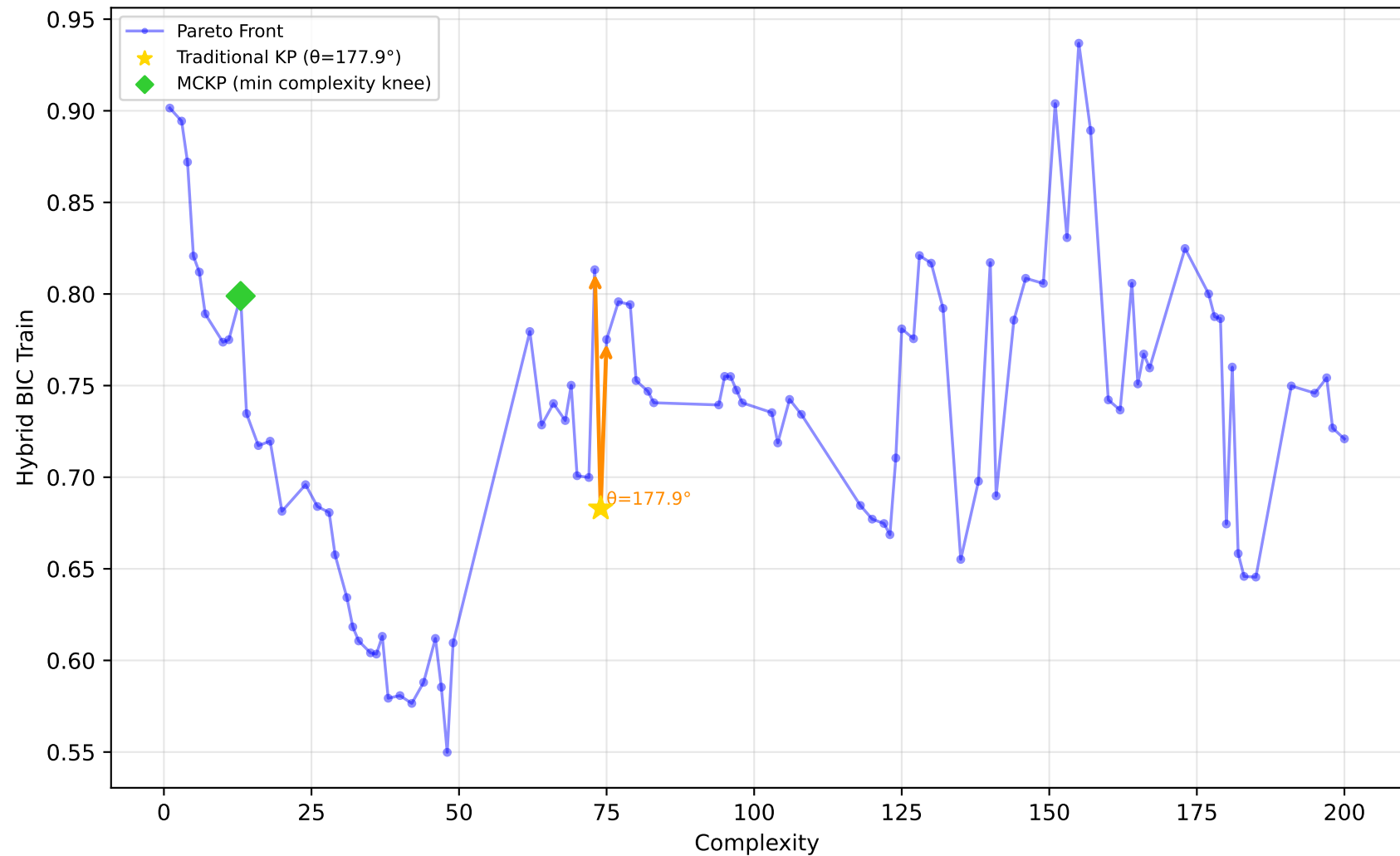
542_pollution - Run 15 - SVP - Hybrid BIC Train \lambda_1=0.00, \lambda_2=0.00, \lambda_3=0.20 | Difficulty: 0.42 | Method: mckp
