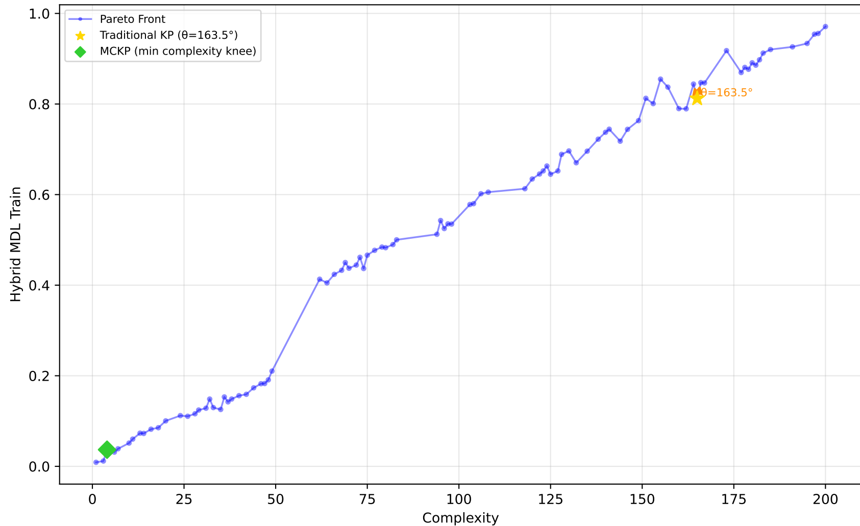
542_pollution - Run 15 - SVP - Hybrid MDL Train \lambda_1=0.00, \lambda_2=0.00, \lambda_3=0.20 | Difficulty: 0.42 | Method: mckp
