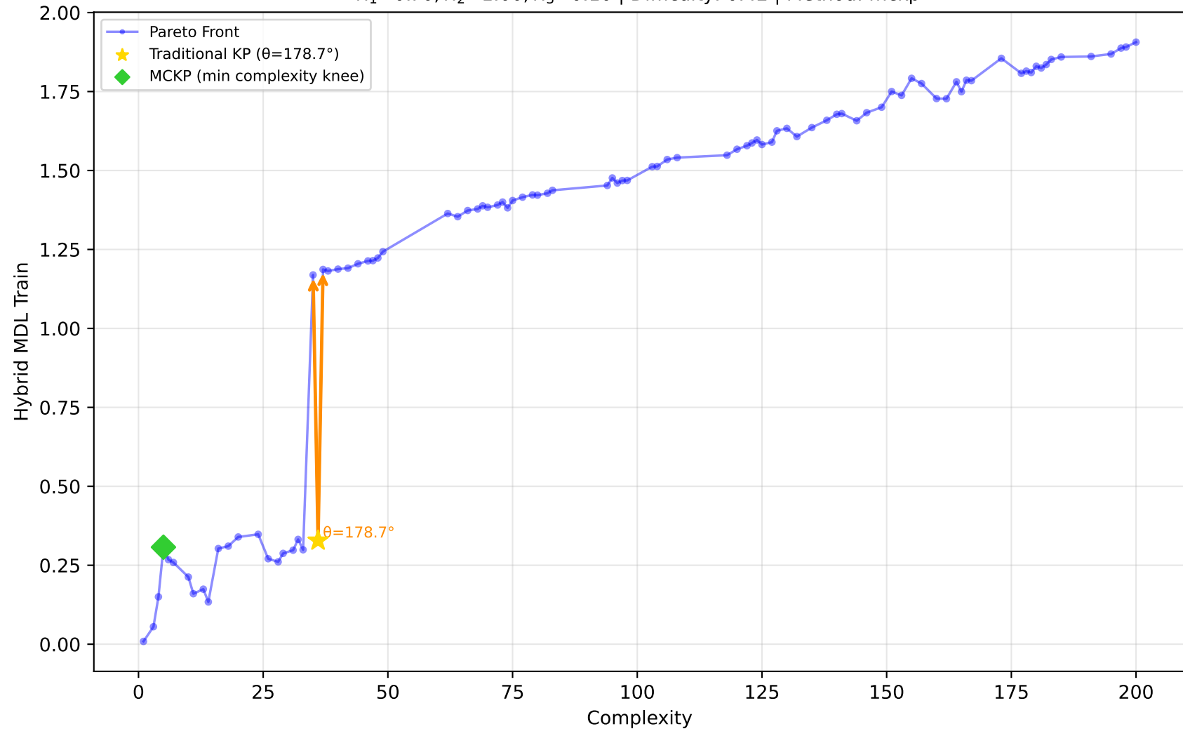
542_pollution - Run 15 - SVP - Hybrid MDL Train \lambda_1=0.70, \lambda_2=1.00, \lambda_3=0.10 | Difficulty: 0.42 | Method: mckp
