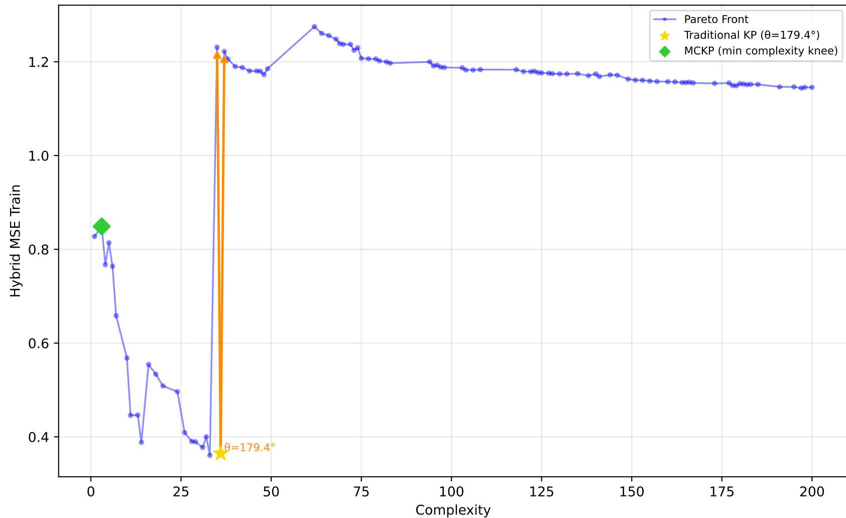
542_pollution - Run 15 - SVP - Hybrid MSE Train \lambda_1=0.70, \lambda_2=1.00, \lambda_3=0.10 | Difficulty: 0.42 | Method: mckp
