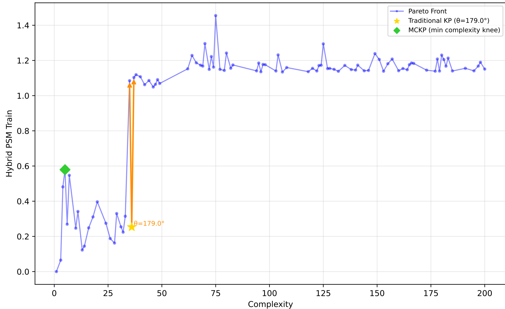
542_pollution - Run 15 - SVP - Hybrid PSM Train \lambda_1=0.70 , \lambda_2=1.00 , \lambda_3=0.10 | Difficulty: 0.42 | Method: mckp
