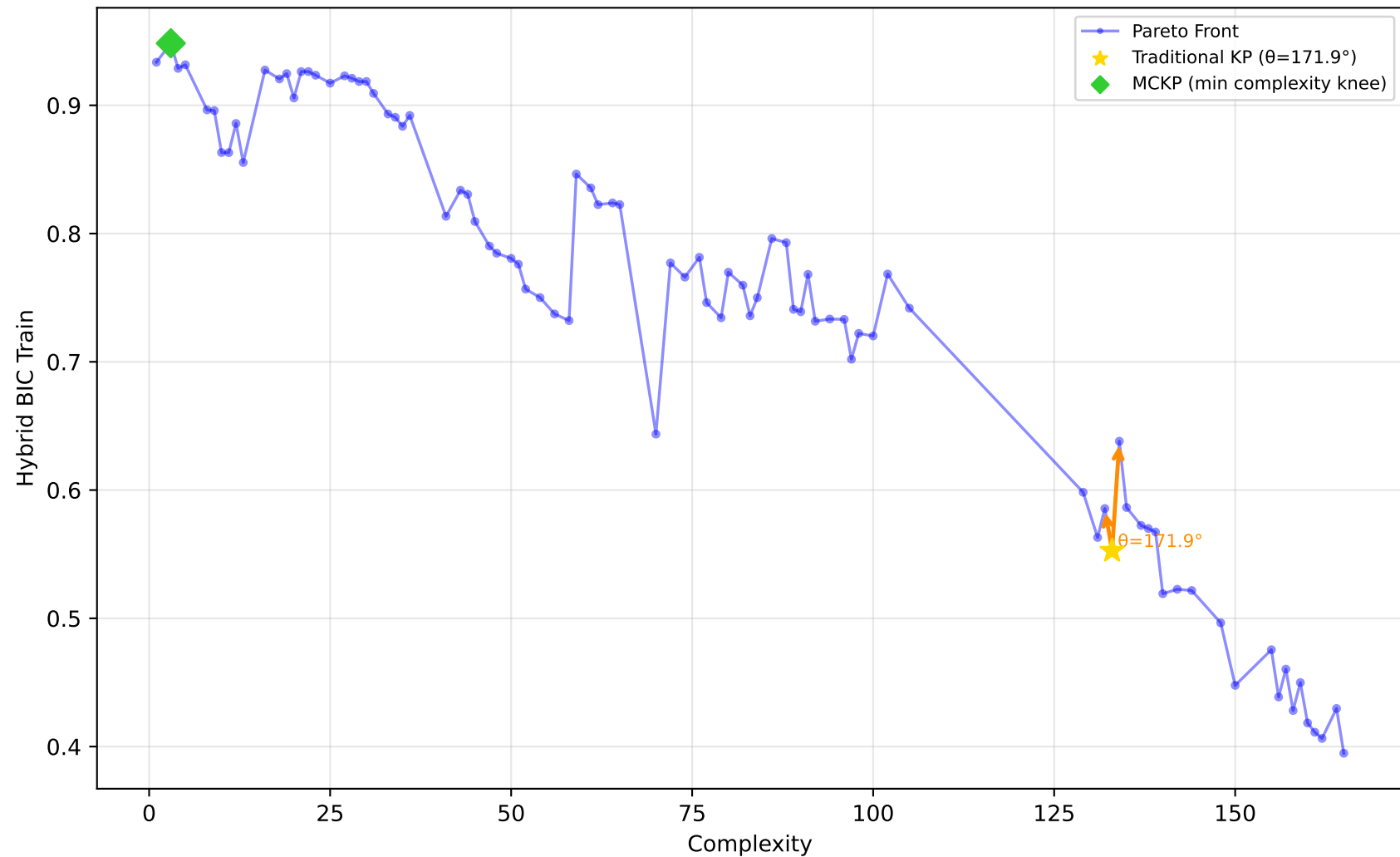
542_pollution - Run 16 - MVP - Hybrid BIC Train \lambda_1=0.40, \lambda_2=0.10, \lambda_3=0.00 | Difficulty: 0.49 | Method: mckp
