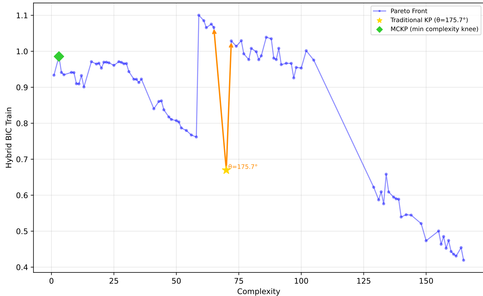
542_pollution - Run 16 - MVP - Hybrid BIC Train \lambda_1=1.00, \lambda_2=0.10, \lambda_3=0.00 | Difficulty: 0.49 | Method: mckp
