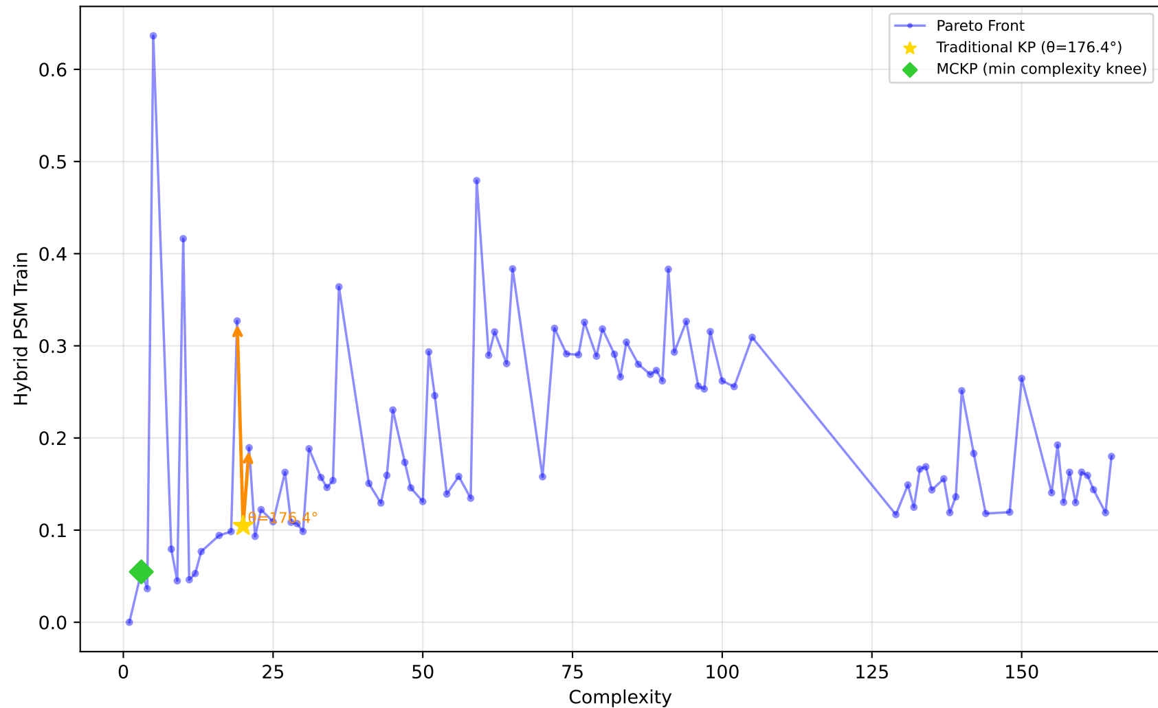
542_pollution - Run 16 - MVP - Hybrid PSM Train \lambda_1=0.40, \lambda_2=0.10, \lambda_3=0.00 | Difficulty: 0.49 | Method: mckp
