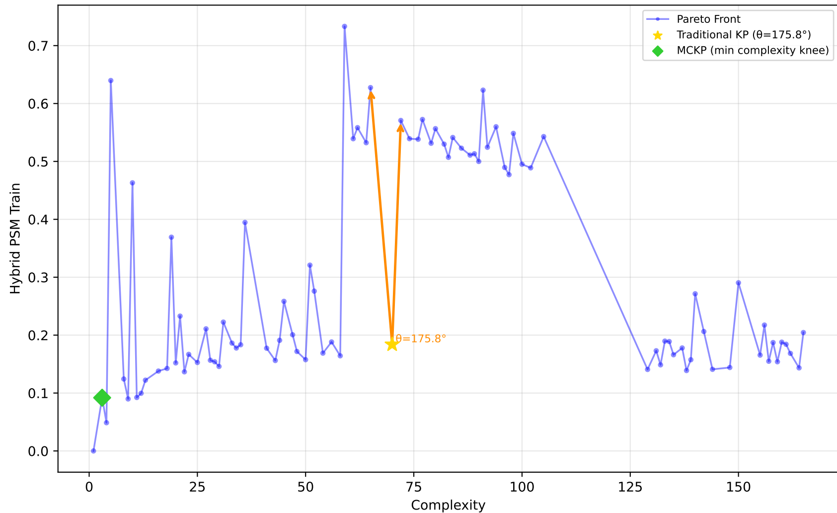
542_pollution - Run 16 - MVP - Hybrid PSM Train \lambda_1=1.00, \lambda_2=0.10, \lambda_3=0.00 | Difficulty: 0.49 | Method: mckp
