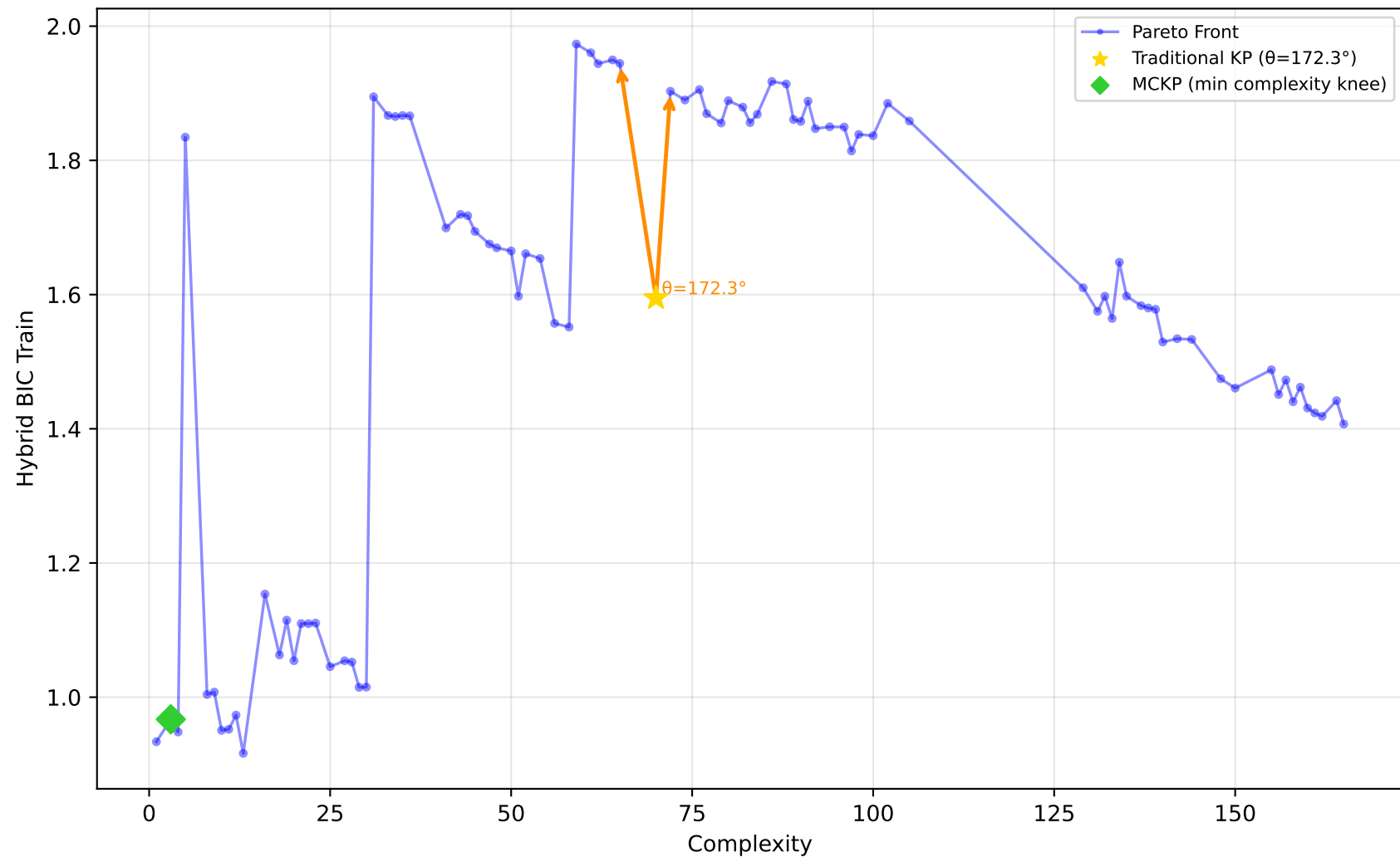
542_pollution - Run 16 - SVP - Hybrid BIC Train \lambda_1=0.70 , \lambda_2=1.00 , \lambda_3=0.10 | Difficulty: 0.49 | Method: mckp
