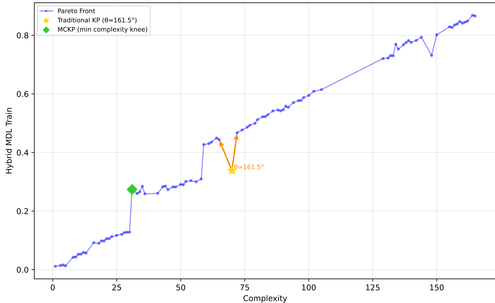
542_pollution - Run 16 - SVP - Hybrid MDL Train \lambda_1=0.00, \lambda_2=0.00, \lambda_3=0.20 | Difficulty: 0.49 | Method: mckp
