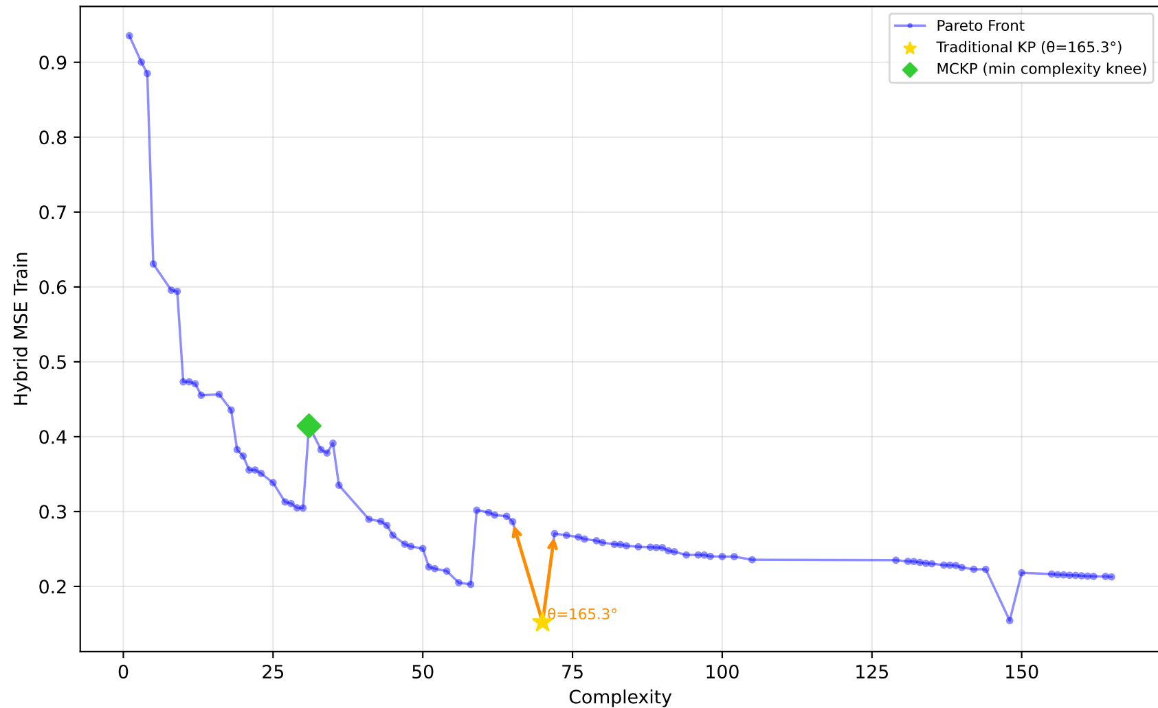
542_pollution - Run 16 - SVP - Hybrid MSE Train \lambda_1=0.00, \lambda_2=0.00, \lambda_3=0.20 | Difficulty: 0.49 | Method: mckp
