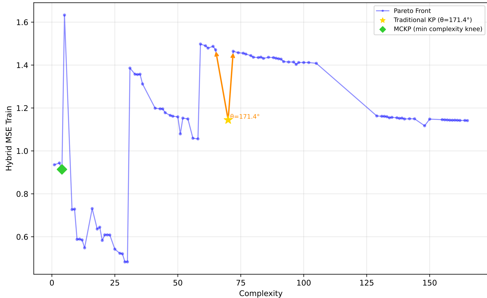
542_pollution - Run 16 - SVP - Hybrid MSE Train \lambda_1=0.70, \lambda_2=1.00, \lambda_3=0.10 | Difficulty: 0.49 | Method: mckp
