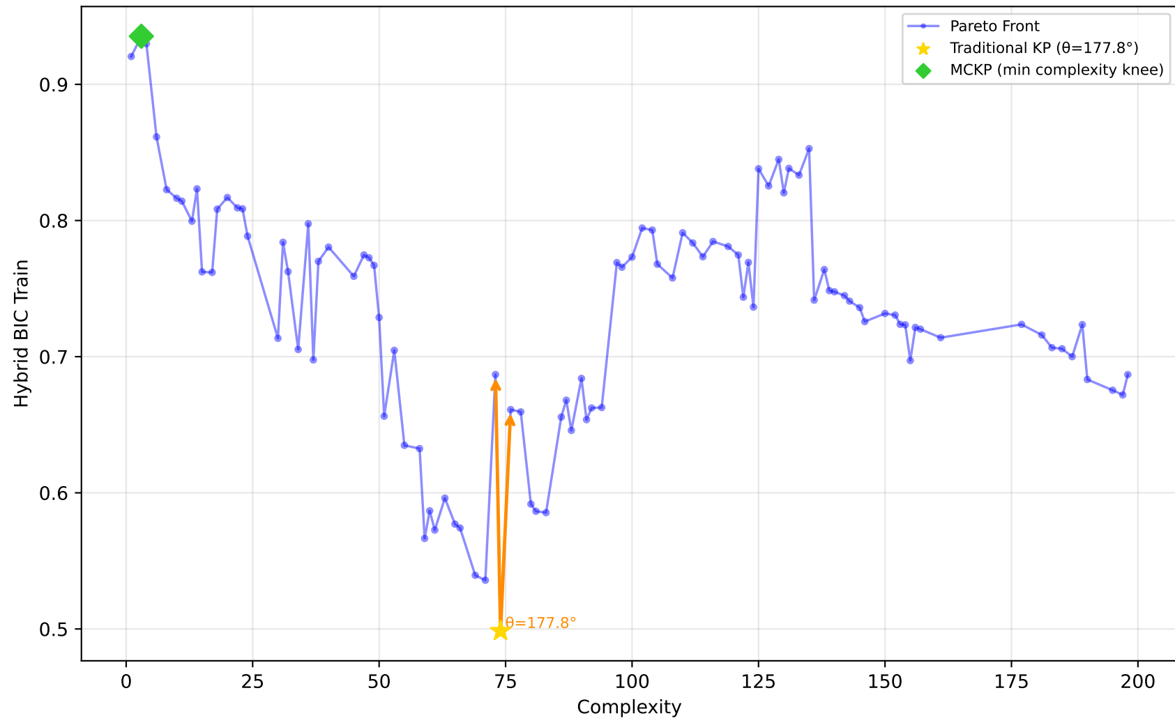
542_pollution - Run 17 - MVP - Hybrid BIC Train \lambda_1=0.40, \lambda_2=0.10, \lambda_3=0.00 | Difficulty: 0.13 | Method: mckp
