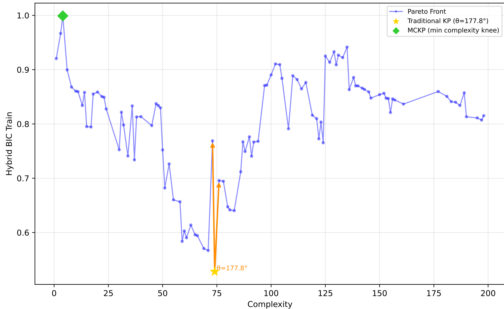
542_pollution - Run 17 - MVP - Hybrid BIC Train \lambda_1=1.00, \lambda_2=0.10, \lambda_3=0.00 | Difficulty: 0.13 | Method: mckp
