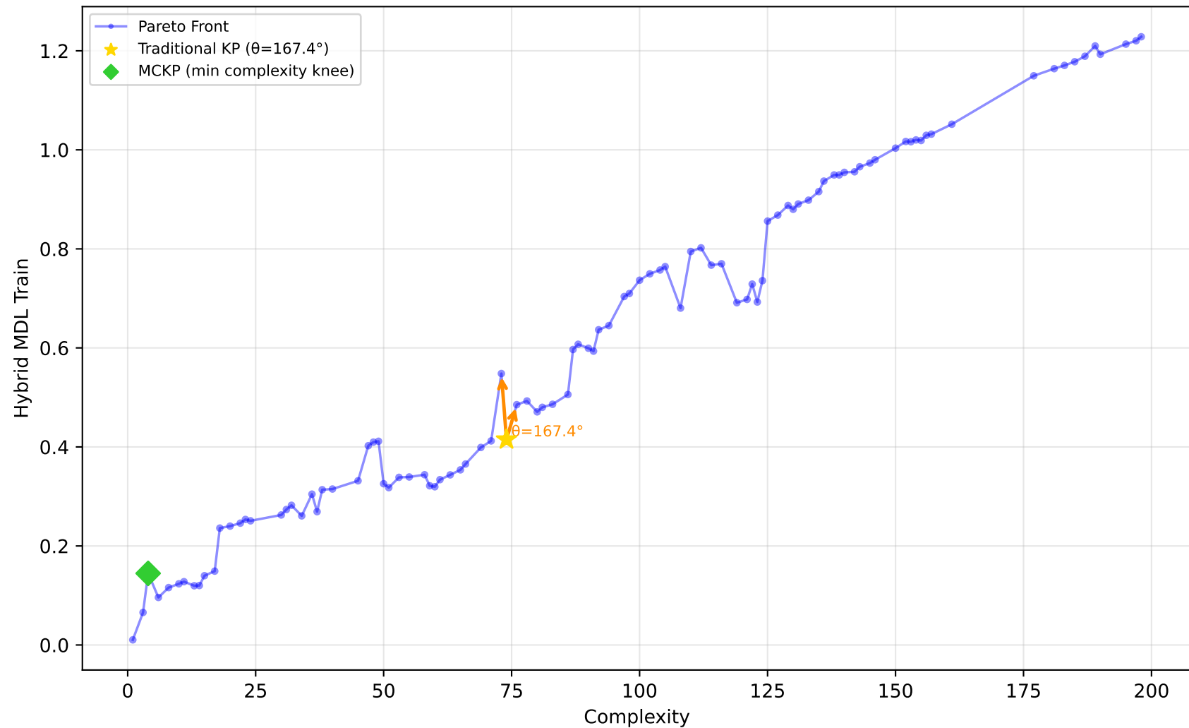
542_pollution - Run 17 - MVP - Hybrid MDL Train \lambda_1=1.00, \lambda_2=0.10, \lambda_3=0.00 | Difficulty: 0.13 | Method: mckp
