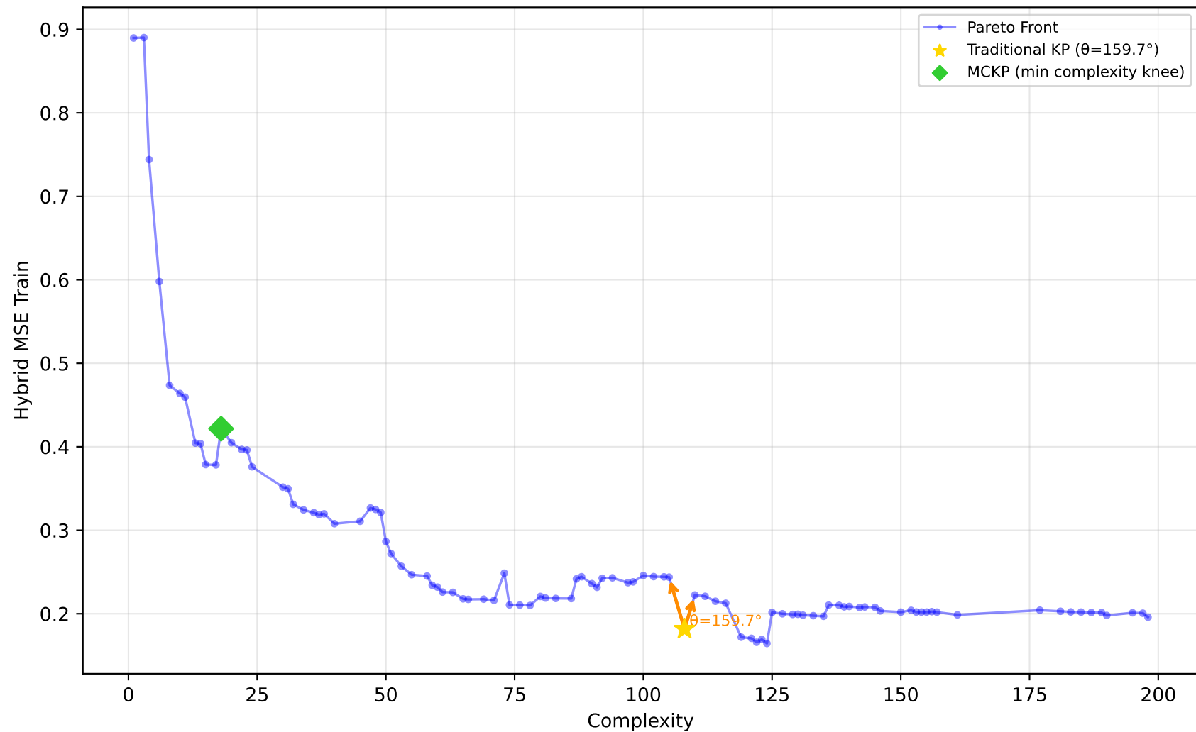
542_pollution - Run 17 - MVP - Hybrid MSE Train \lambda_1=0.40, \lambda_2=0.10, \lambda_3=0.00 | Difficulty: 0.13 | Method: mckp
