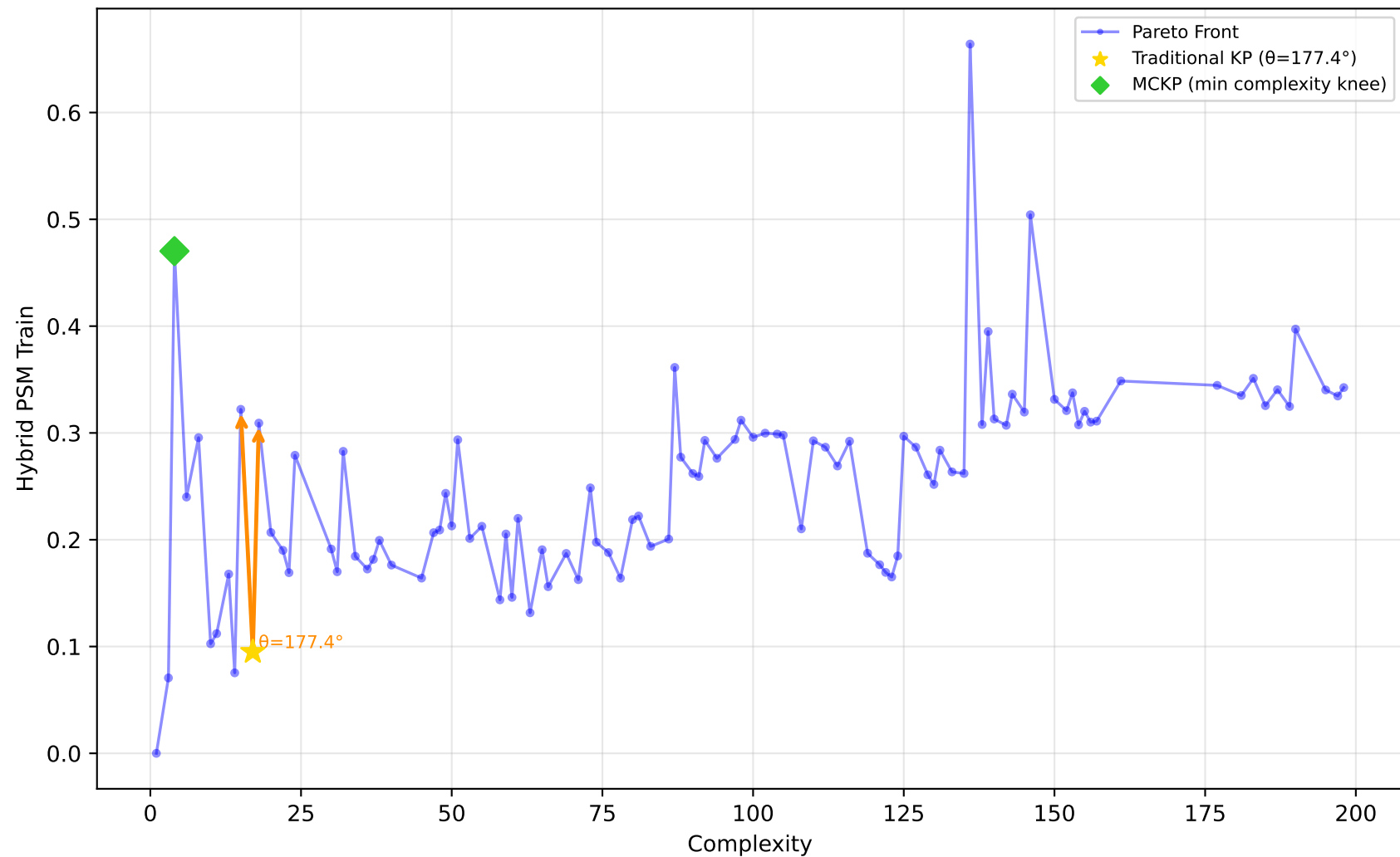
542_pollution - Run 17 - MVP - Hybrid PSM Train \lambda_1=1.00, \bar{\lambda}_2=0.10, \lambda_3=0.00 | Difficulty: 0.13 | Method: mckp
