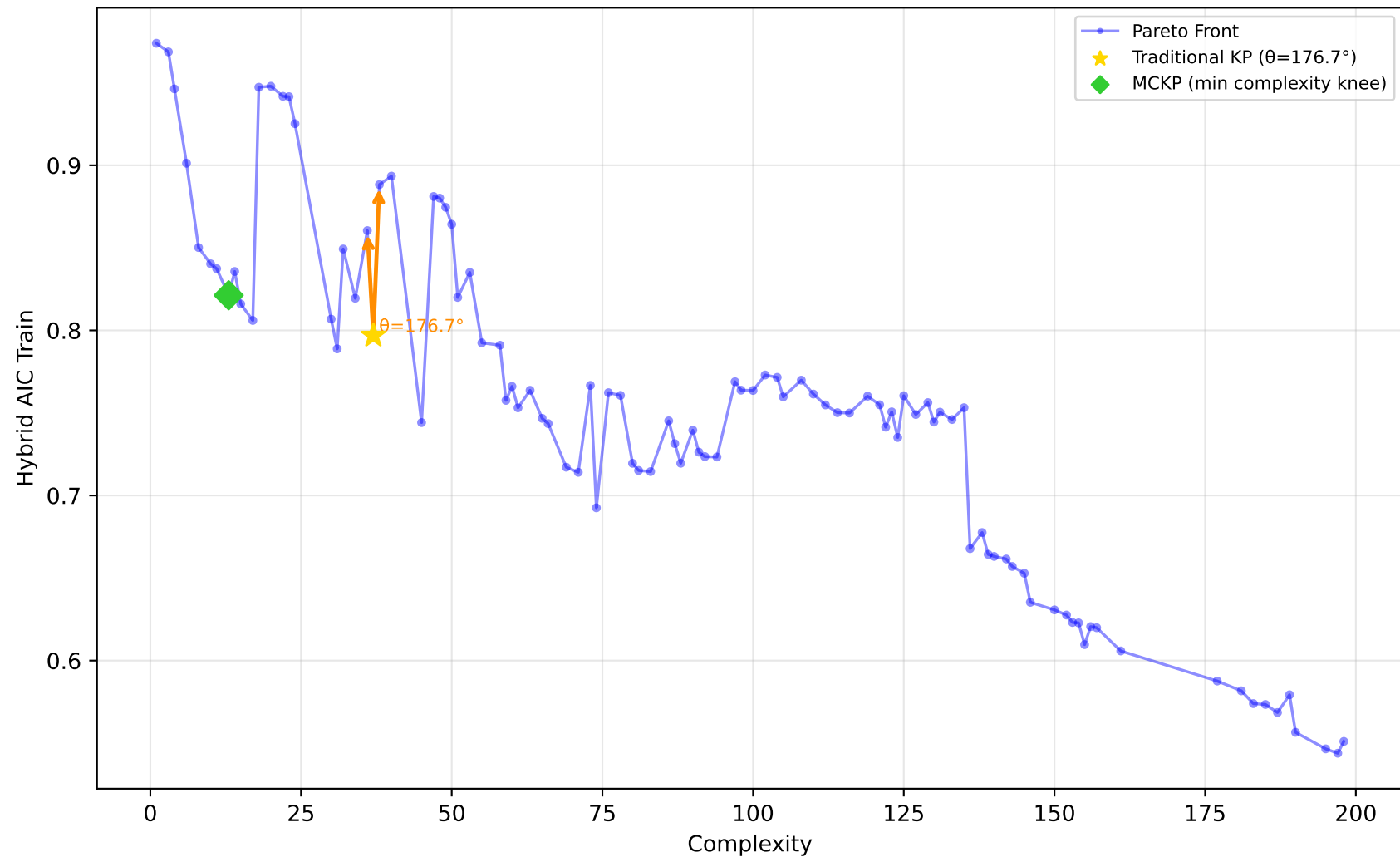
542_pollution - Run 17 - SVP - Hybrid AIC Train \lambda_1=0.00, \lambda_2=0.00, \lambda_3=0.20 | Difficulty: 0.13 | Method: mckp
