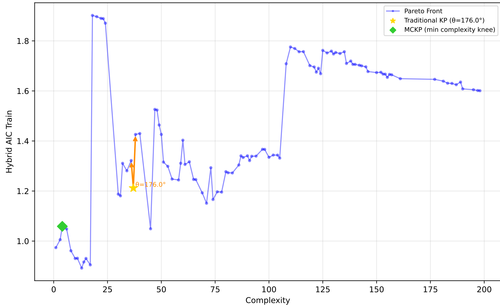
542_pollution - Run 17 - SVP - Hybrid AIC Train \lambda_1=0.70 , \lambda_2=1.00 , \lambda_3=0.10 | Difficulty: 0.13 | Method: mckp
