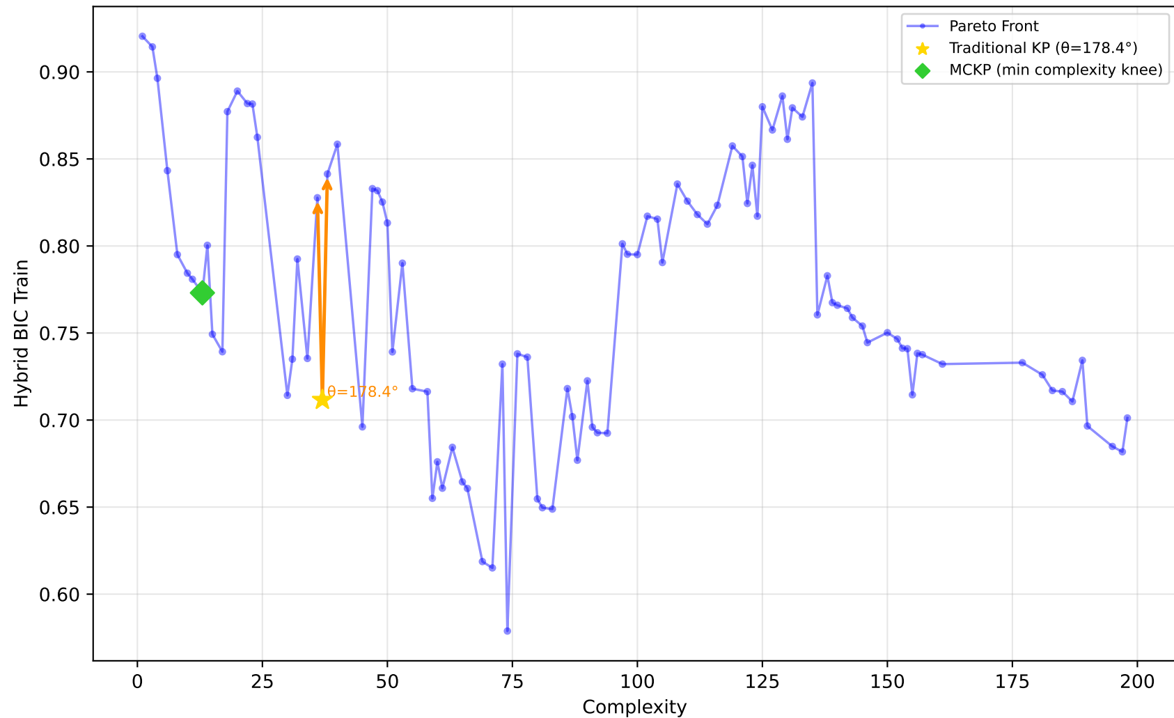
542_pollution - Run 17 - SVP - Hybrid BIC Train \lambda_1=0.00, \lambda_2=0.00, \lambda_3=0.20 | Difficulty: 0.13 | Method: mckp
