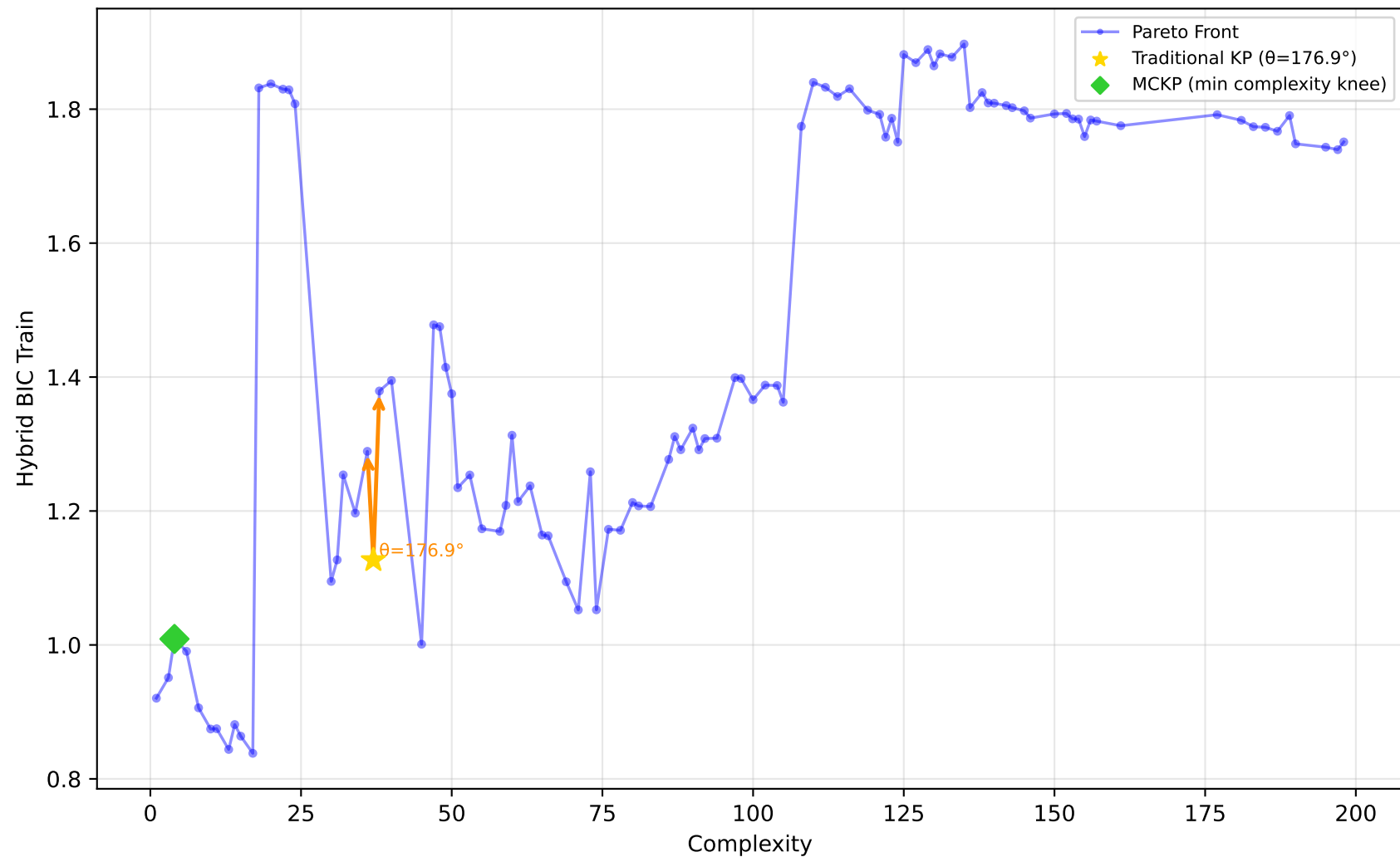
542_pollution - Run 17 - SVP - Hybrid BIC Train \lambda_1=0.70, \lambda_2=1.00, \lambda_3=0.10 | Difficulty: 0.13 | Method: mckp
