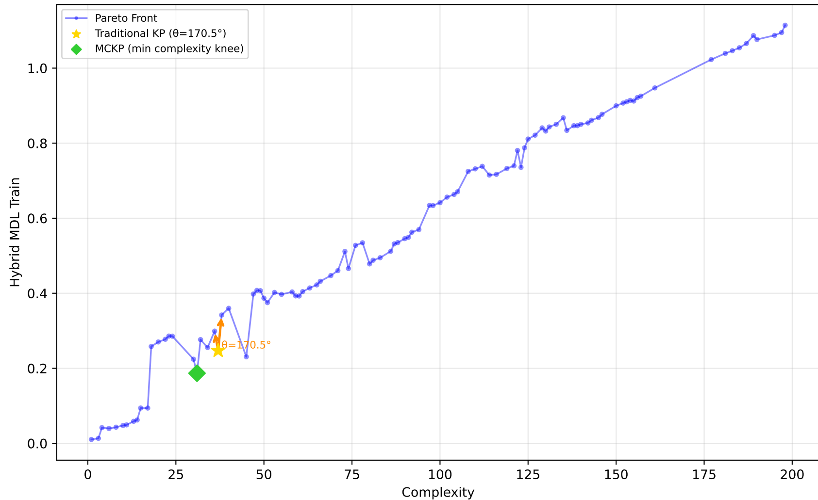
542_pollution - Run 17 - SVP - Hybrid MDL Train \lambda_1=0.00, \lambda_2=0.00, \lambda_3=0.20 | Difficulty: 0.13 | Method: mckp
