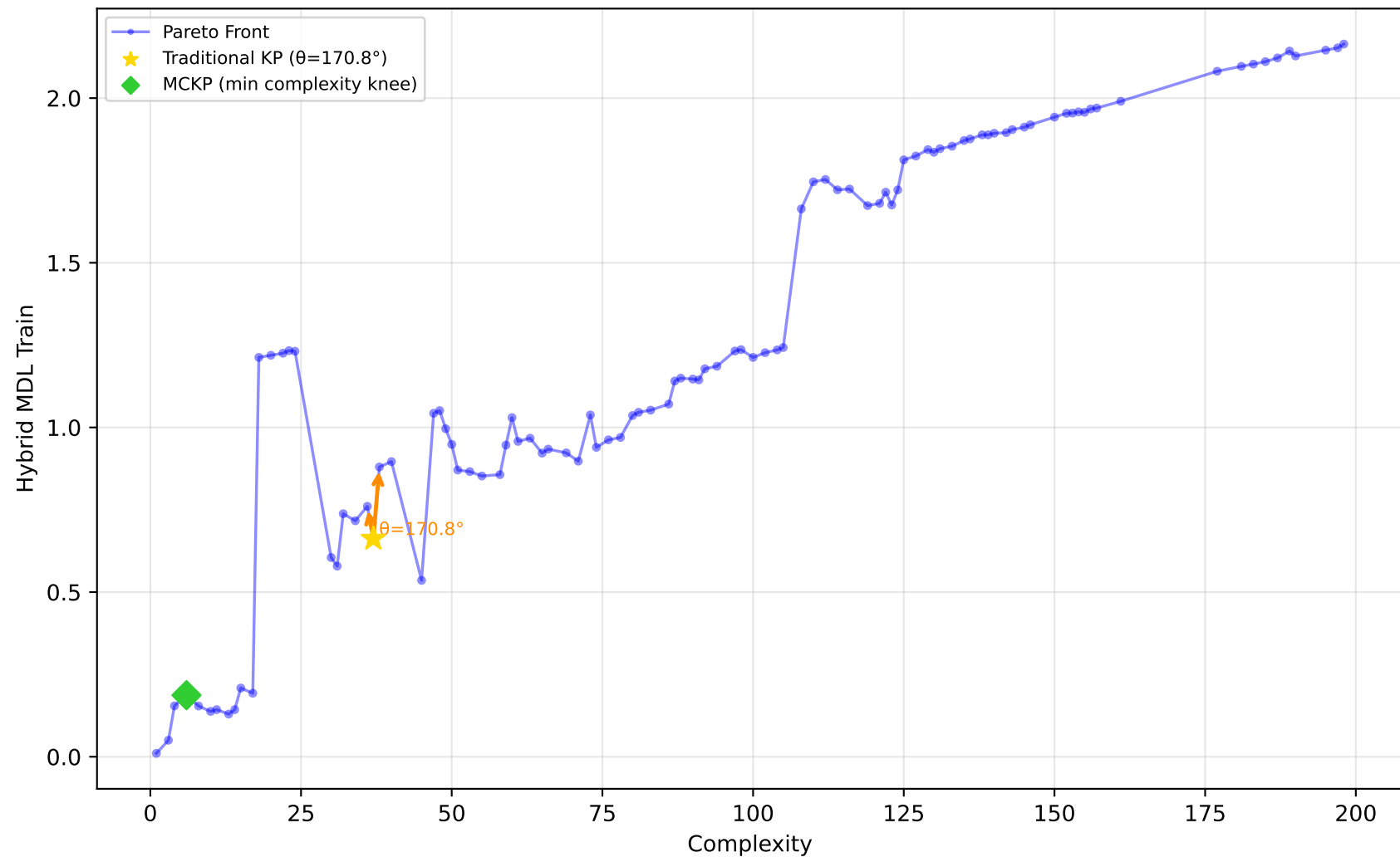
542_pollution - Run 17 - SVP - Hybrid MDL Train \lambda_1=0.70 , \lambda_2=1.00 , \lambda_3=0.10 | Difficulty: 0.13 | Method: mckp
