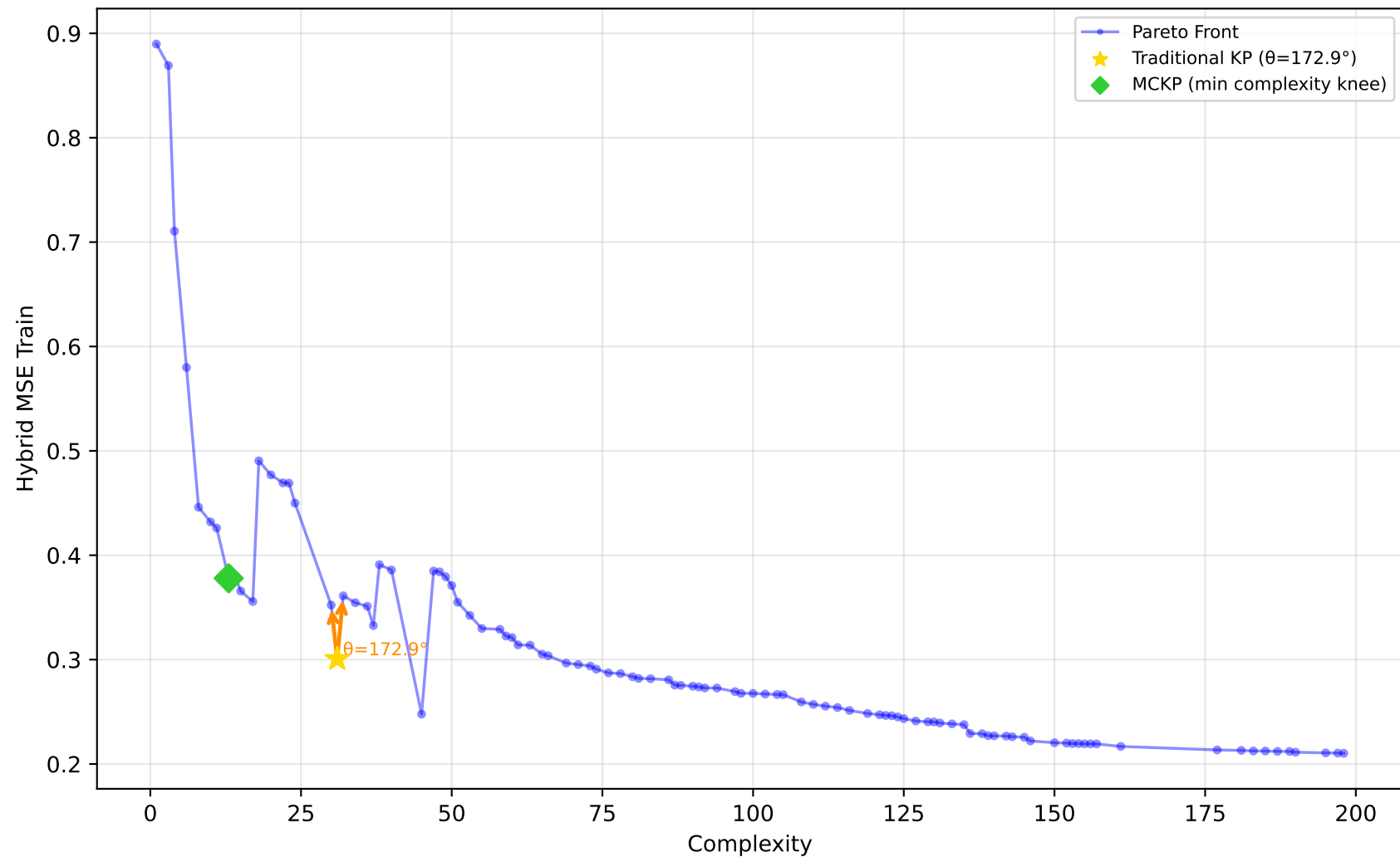
542_pollution - Run 17 - SVP - Hybrid MSE Train \lambda_1=0.00, \lambda_2=0.00, \lambda_3=0.20 | Difficulty: 0.13 | Method: mckp
