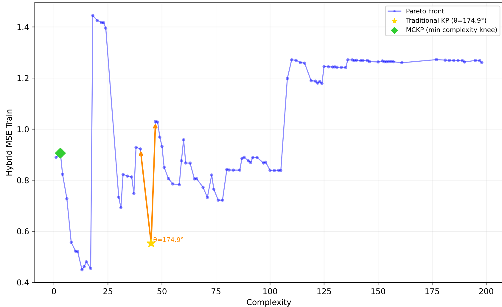
542_pollution - Run 17 - SVP - Hybrid MSE Train \lambda_1=0.70, \lambda_2=1.00, \lambda_3=0.10 | Difficulty: 0.13 | Method: mckp
