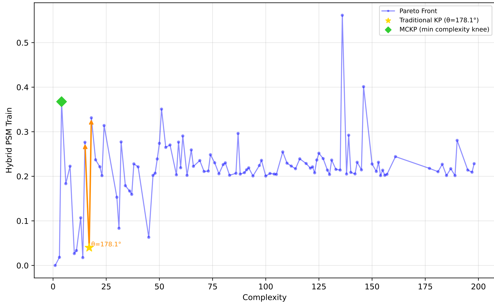
542_pollution - Run 17 - SVP - Hybrid PSM Train \lambda_1=0.00, \lambda_2=0.00, \lambda_3=0.20 | Difficulty: 0.13 | Method: mckp
