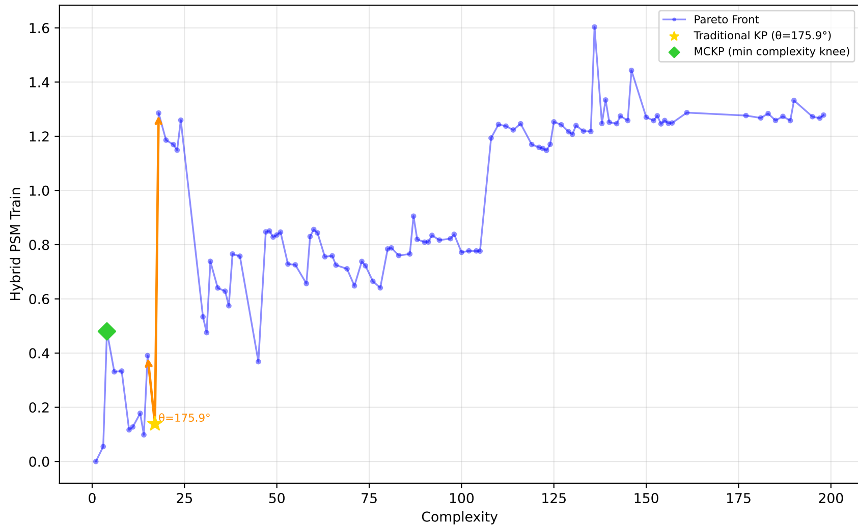
542_pollution - Run 17 - SVP - Hybrid PSM Train \lambda_1=0.70, \lambda_2=1.00, \lambda_3=0.10 | Difficulty: 0.13 | Method: mckp
