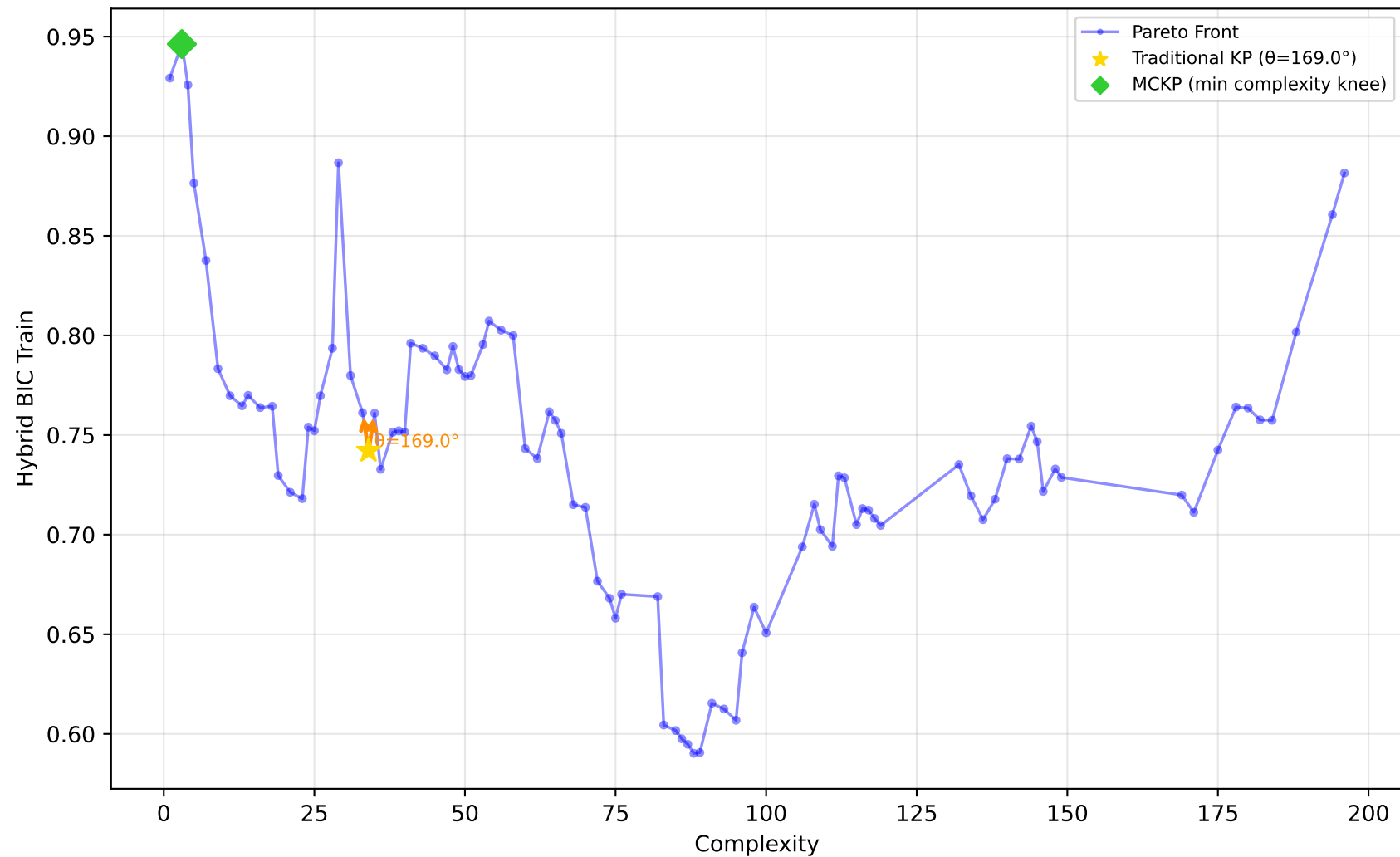
542_pollution - Run 18 - MVP - Hybrid BIC Train \lambda_1=0.40, \lambda_2=0.10, \lambda_3=0.00 | Difficulty: 0.55 | Method: mckp
