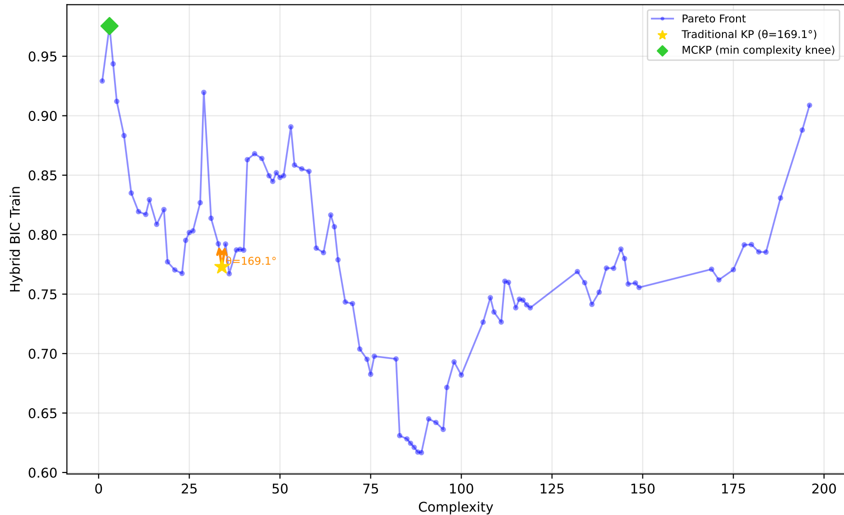
542_pollution - Run 18 - MVP - Hybrid BIC Train \lambda_1=1.00, \lambda_2=0.10, \lambda_3=0.00 | Difficulty: 0.55 | Method: mckp
