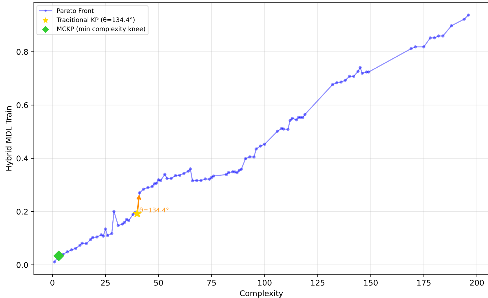
542_pollution - Run 18 - MVP - Hybrid MDL Train \lambda_1=0.40, \lambda_2=0.10, \lambda_3=0.00 | Difficulty: 0.55 | Method: mckp
