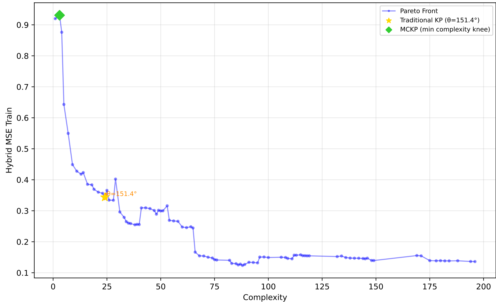
542_pollution - Run 18 - MVP - Hybrid MSE Train \lambda_1=0.40, \lambda_2=0.10, \lambda_3=0.00 | Difficulty: 0.55 | Method: mckp
