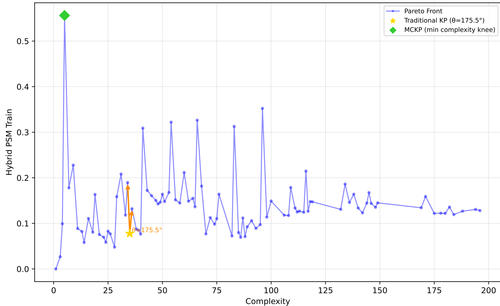
542_pollution - Run 18 - MVP - Hybrid PSM Train \lambda_1=0.40, \lambda_2=0.10, \lambda_3=0.00 | Difficulty: 0.55 | Method: mckp
