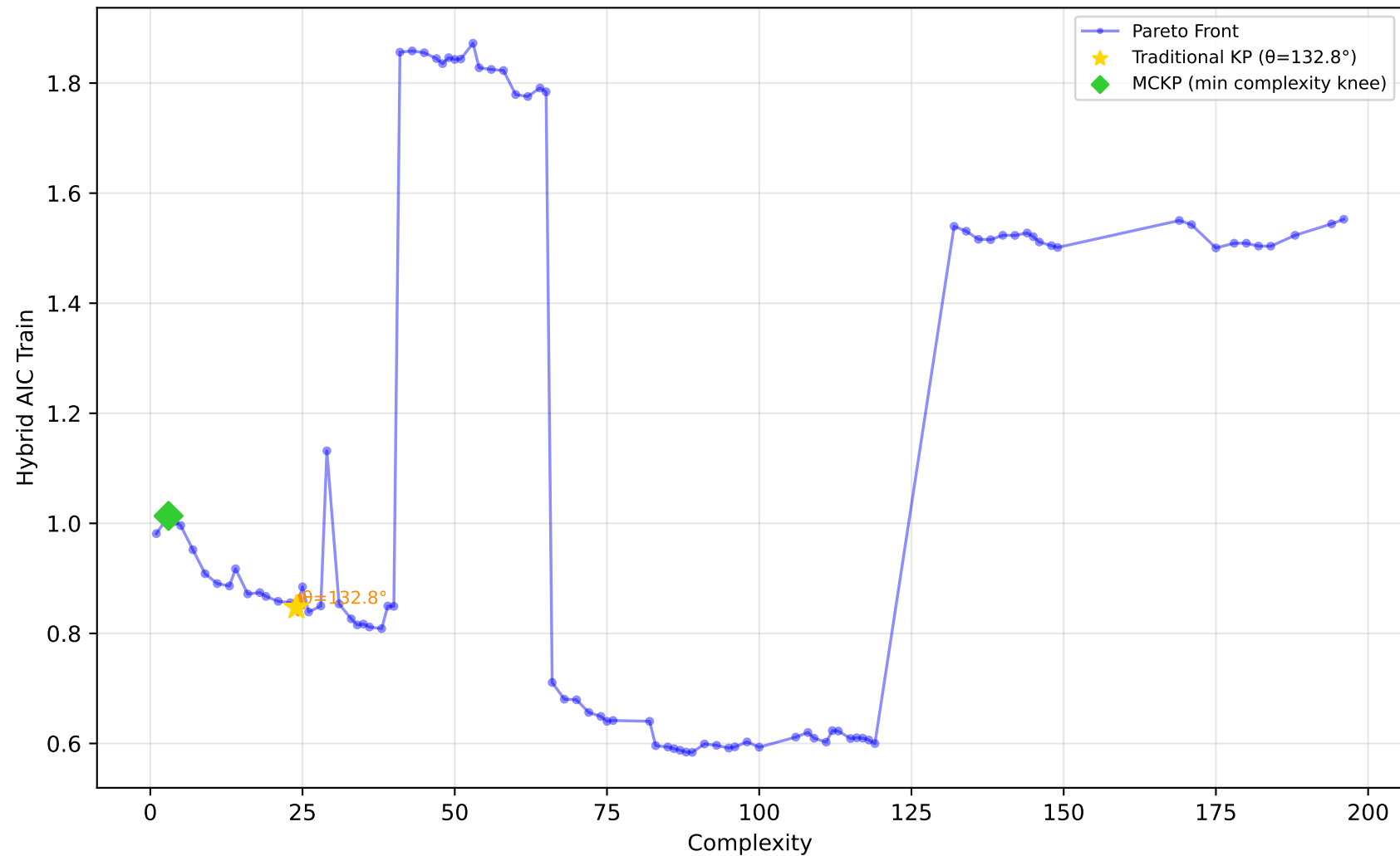
542_pollution - Run 18 - SVP - Hybrid AIC Train \lambda_1=0.70, \lambda_2=1.00, \lambda_3=0.10 | Difficulty: 0.55 | Method: mckp
