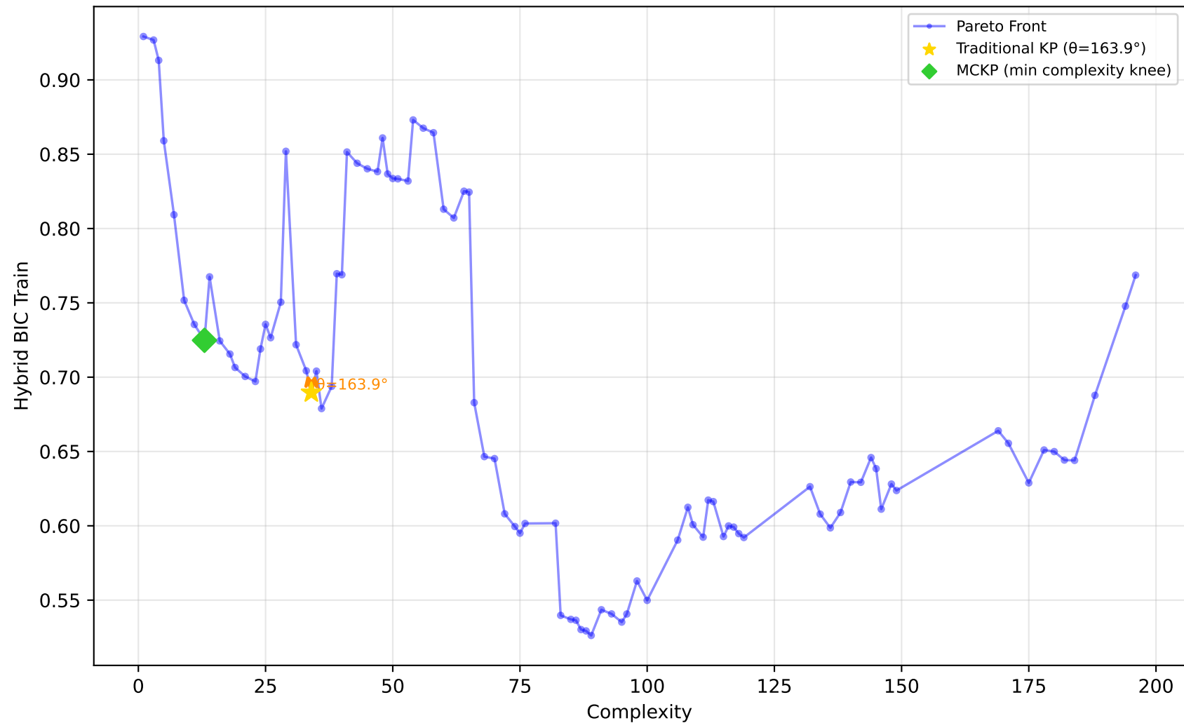
542_pollution - Run 18 - SVP - Hybrid BIC Train \lambda_1=0.00, \lambda_2=0.00, \lambda_3=0.20 | Difficulty: 0.55 | Method: mckp
