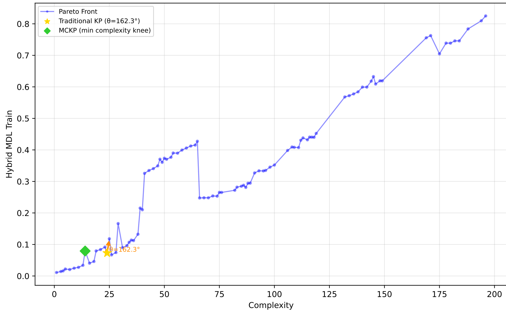
542_pollution - Run 18 - SVP - Hybrid MDL Train \lambda_1=0.00, \lambda_2=0.00, \lambda_3=0.20 | Difficulty: 0.55 | Method: mckp
