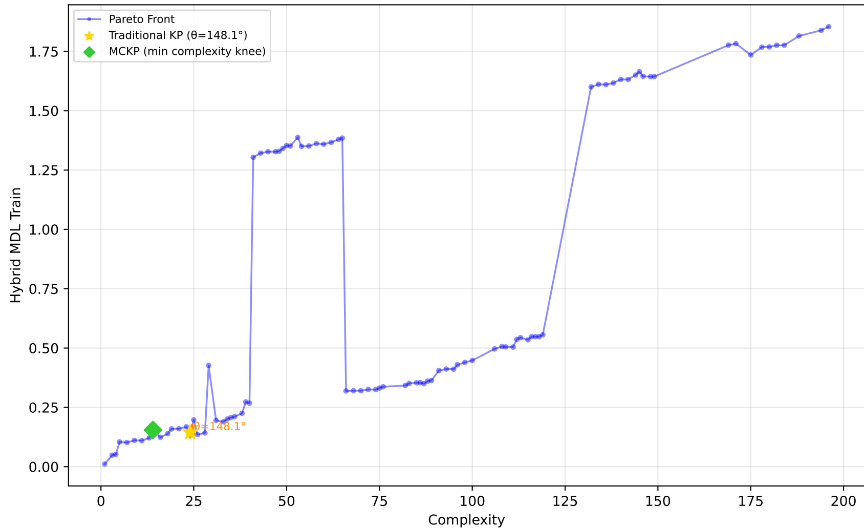
542_pollution - Run 18 - SVP - Hybrid MDL Train \lambda_1=0.70, \lambda_2=1.00, \lambda_3=0.10 | Difficulty: 0.55 | Method: mckp
