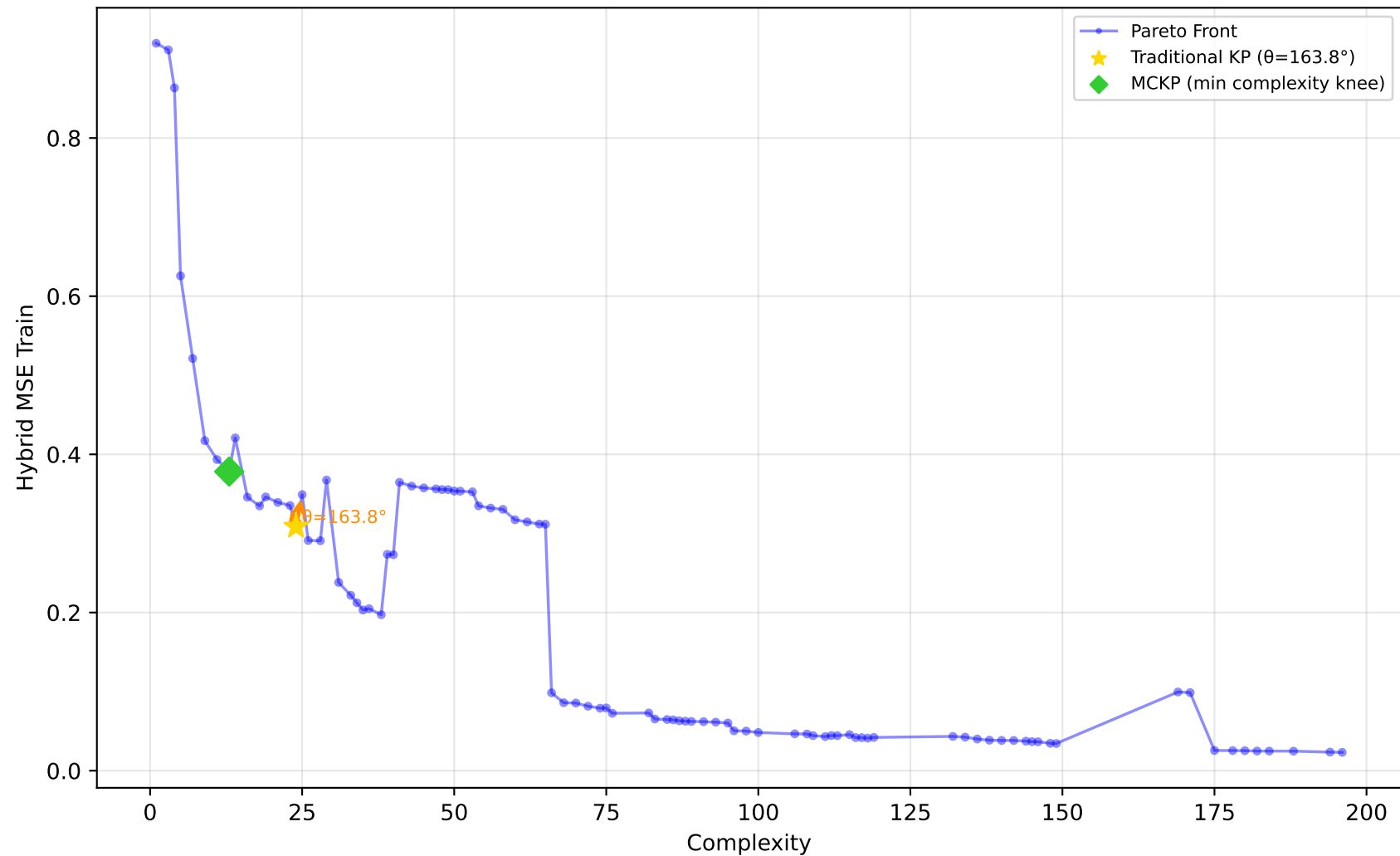
542_pollution - Run 18 - SVP - Hybrid MSE Train \lambda_1=0.00, \lambda_2=0.00, \lambda_3=0.20 | Difficulty: 0.55 | Method: mckp
