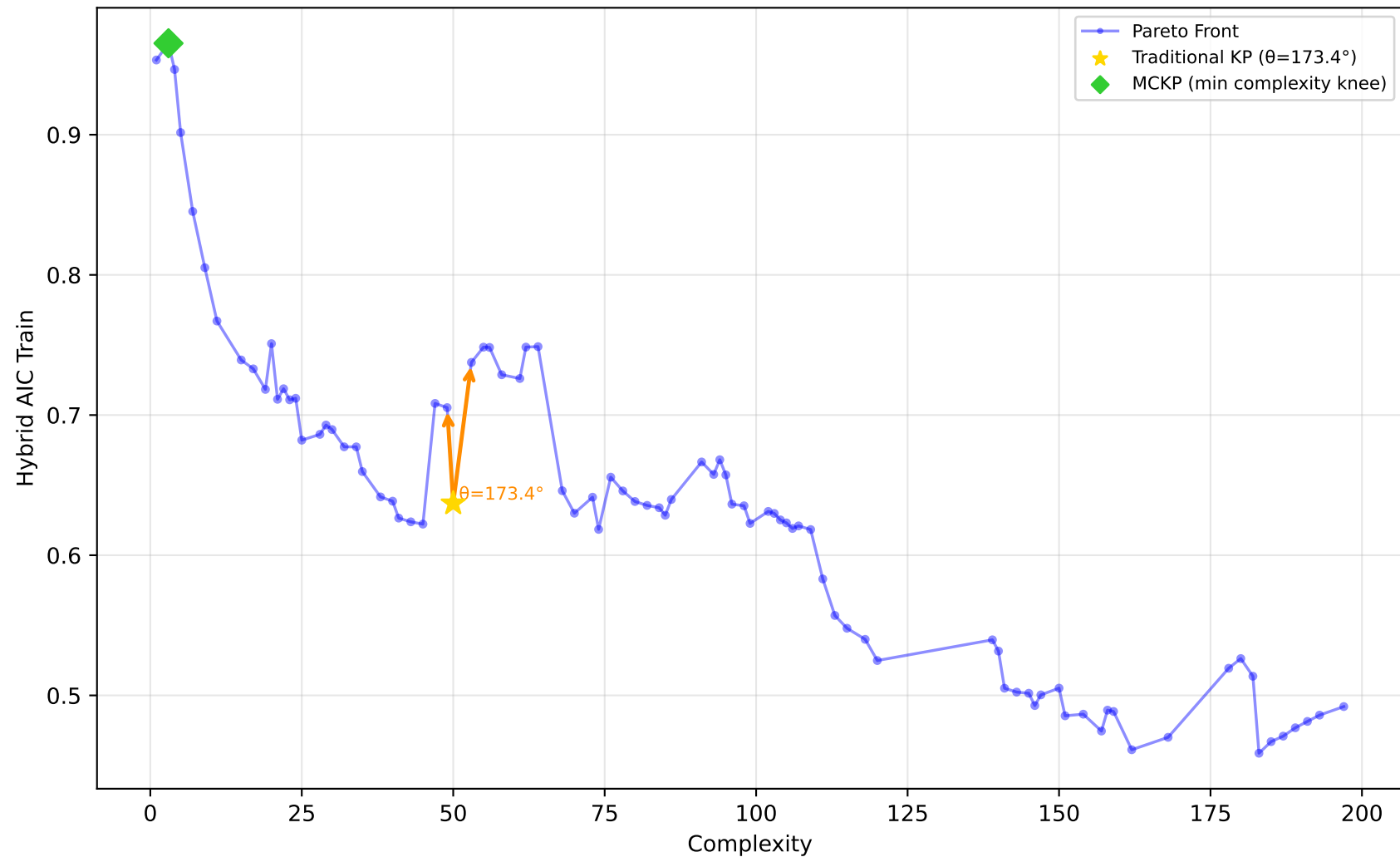
542_pollution - Run 19 - MVP - Hybrid AIC Train \lambda_1=0.40, \lambda_2=0.10, \lambda_3=0.00 | Difficulty: 0.72 | Method: hmr
