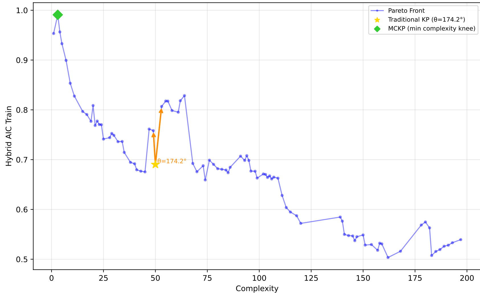
542_pollution - Run 19 - MVP - Hybrid AIC Train \lambda_1=1.00, \lambda_2=0.10, \lambda_3=0.00 | Difficulty: 0.72 | Method: hmr
