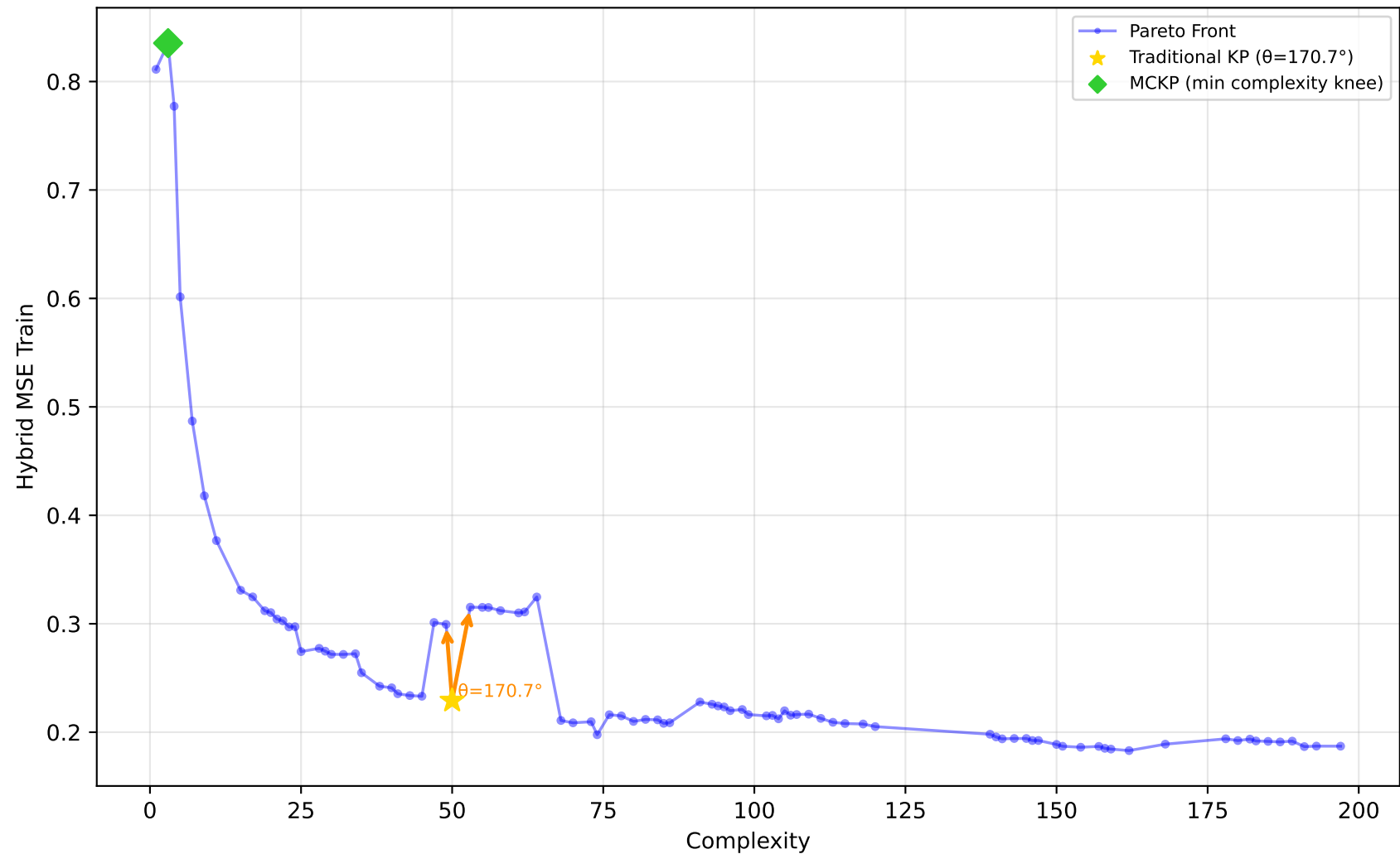
542_pollution - Run 19 - MVP - Hybrid MSE Train \lambda_1=1.00, \lambda_2=0.10, \lambda_3=0.00 | Difficulty: 0.72 | Method: hmr
