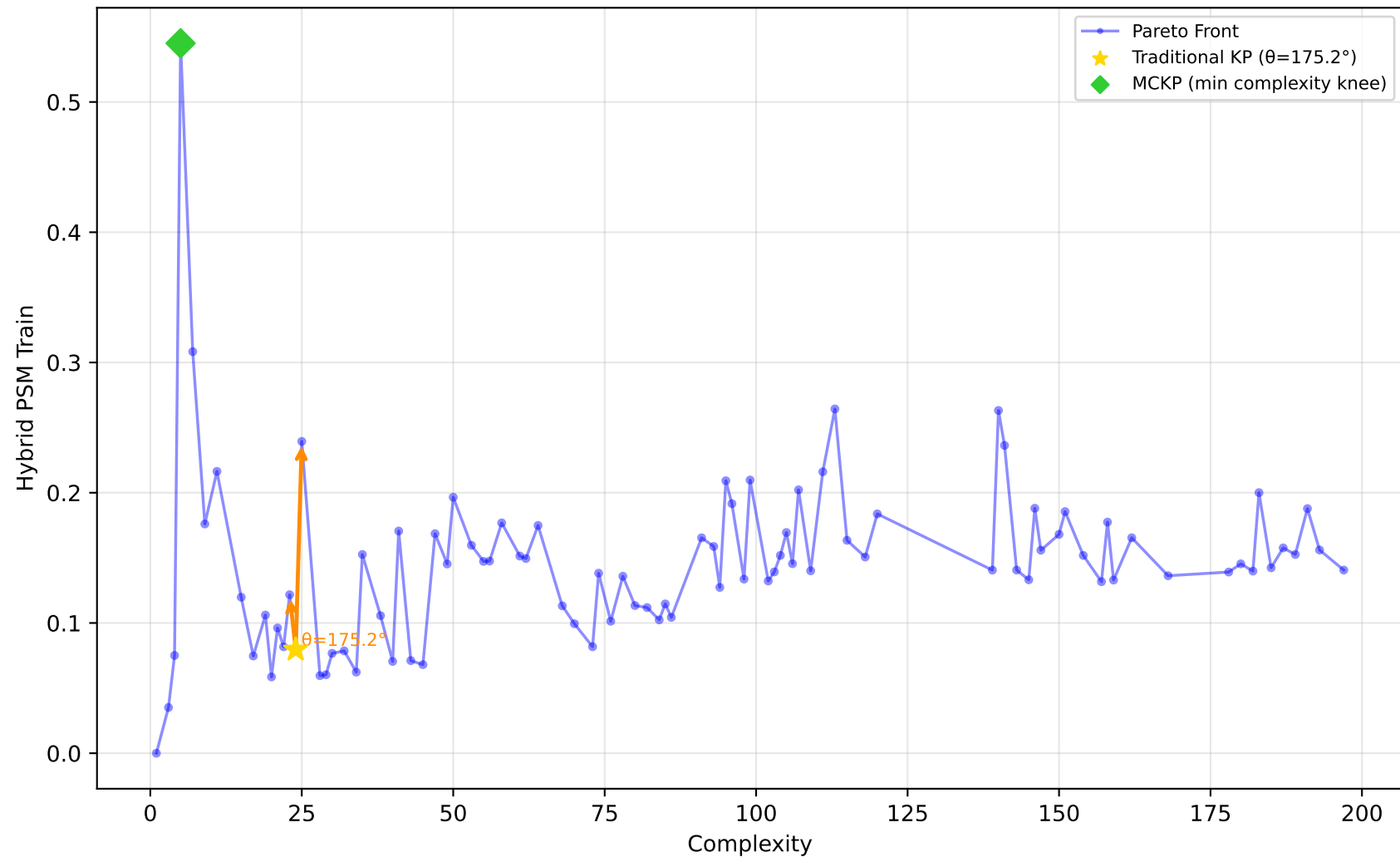
542_pollution - Run 19 - MVP - Hybrid PSM Train \lambda_1=0.40, \lambda_2=0.10, \lambda_3=0.00 | Difficulty: 0.72 | Method: hmr
