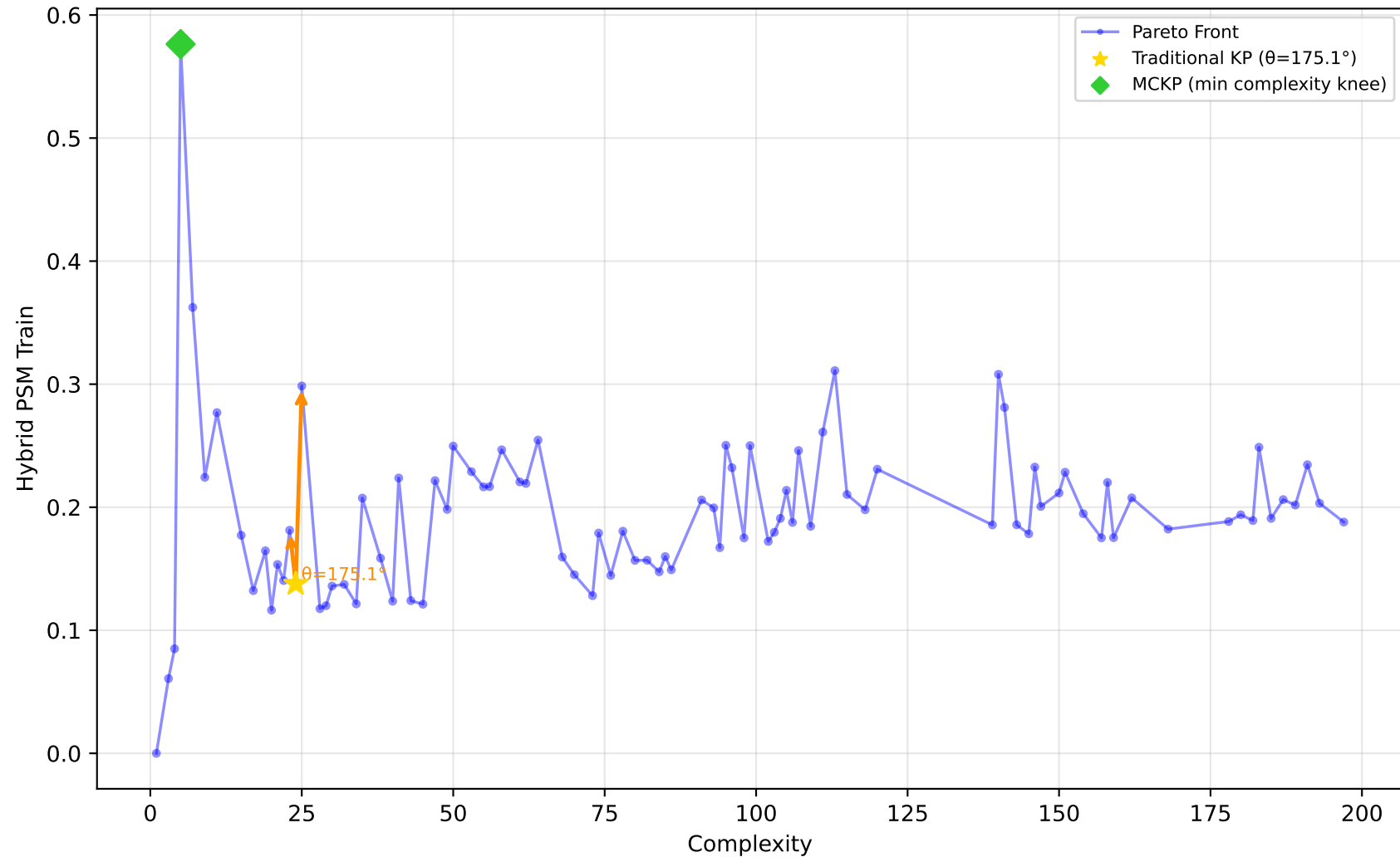
542_pollution - Run 19 - MVP - Hybrid PSM Train \lambda_1=1.00, \lambda_2=0.10, \lambda_3=0.00 | Difficulty: 0.72 | Method: hmr
