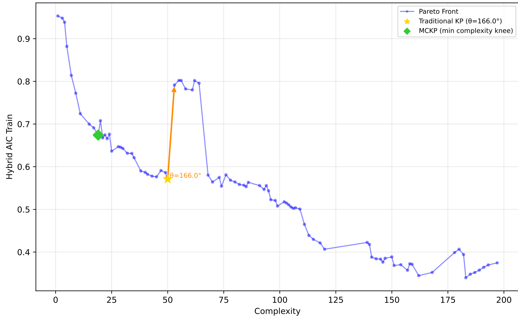
542_pollution - Run 19 - SVP - Hybrid AIC Train \lambda_1=0.00 , \lambda_2=0.00 , \lambda_3=0.20 | Difficulty: 0.72 | Method: hmr
