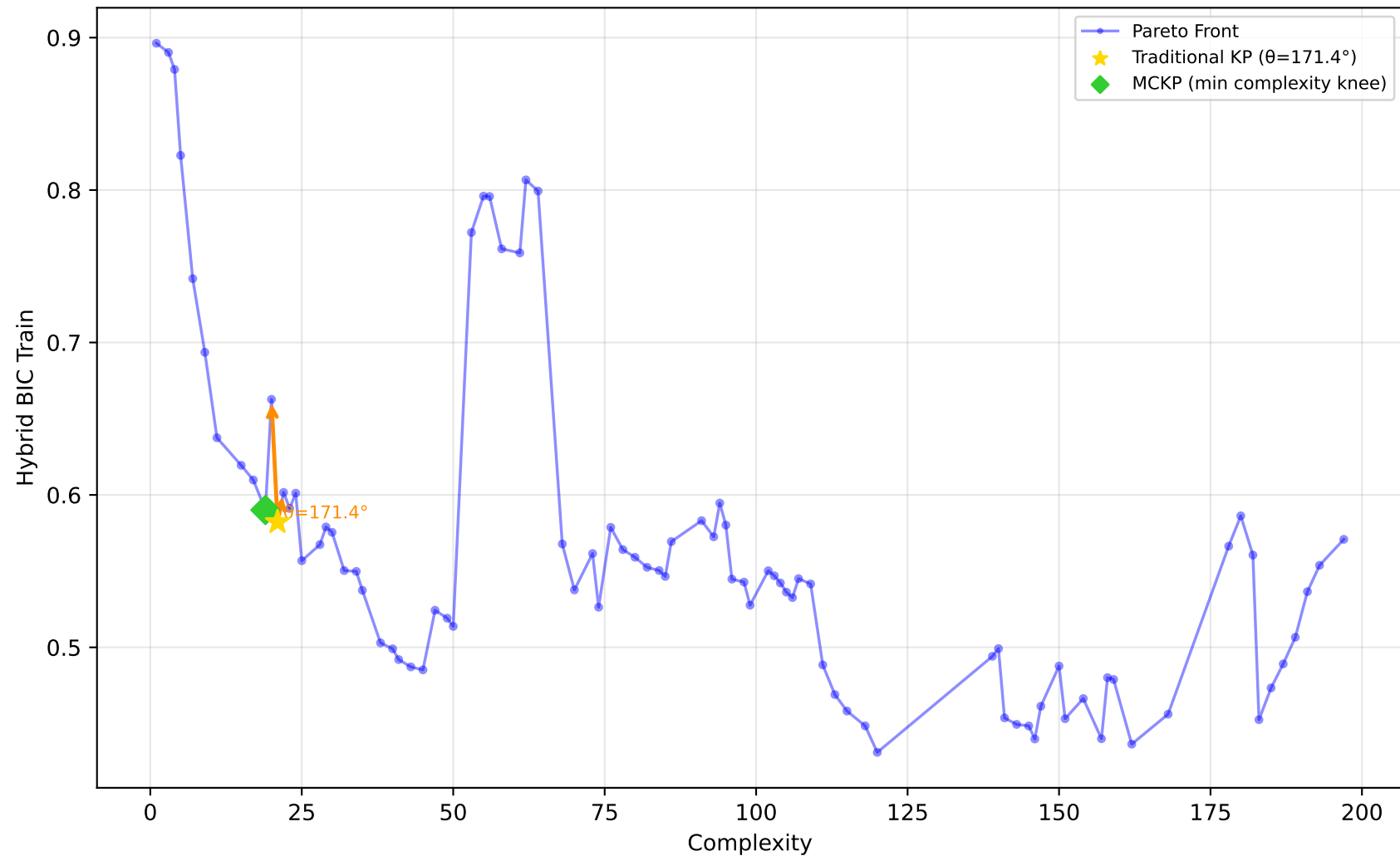
542_pollution - Run 19 - SVP - Hybrid BIC Train \lambda_1=0.00, \bar{\lambda}_2=0.00, \lambda_3=0.20 | Difficulty: 0.72 | Method: hmr
