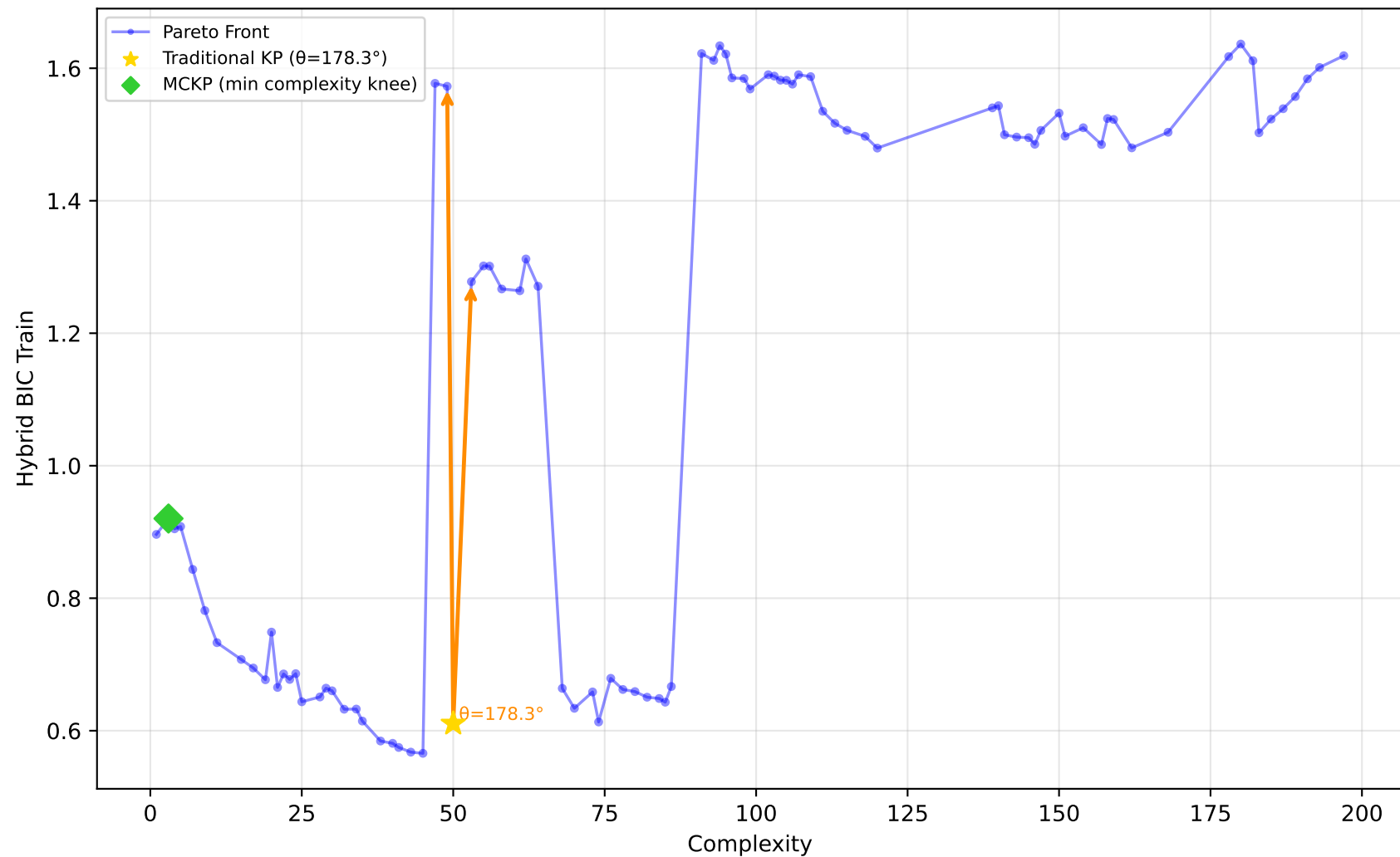
542_pollution - Run 19 - SVP - Hybrid BIC Train \lambda_1=0.70, \lambda_2=1.00, \lambda_3=0.10 | Difficulty: 0.72 | Method: hmr
