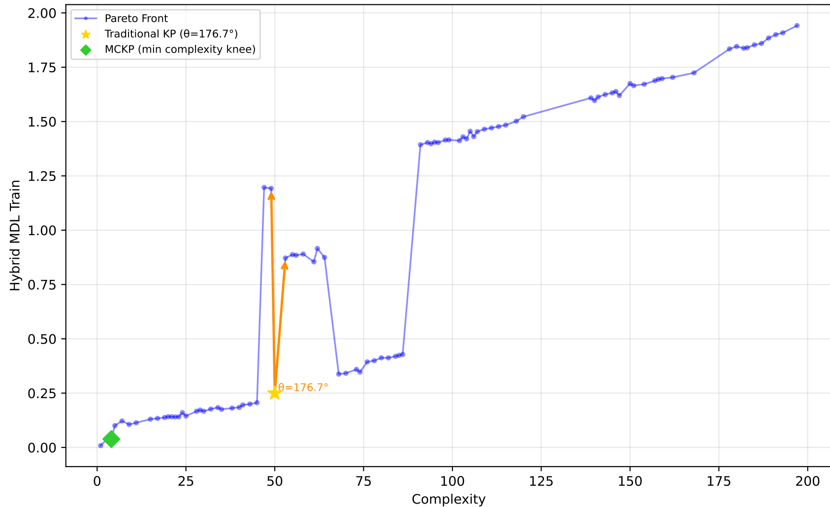
542_pollution - Run 19 - SVP - Hybrid MDL Train \lambda_1=0.70 , \bar{\lambda}_2=1.00 , \lambda_3=0.10 | Difficulty: 0.72 | Method: hmr
