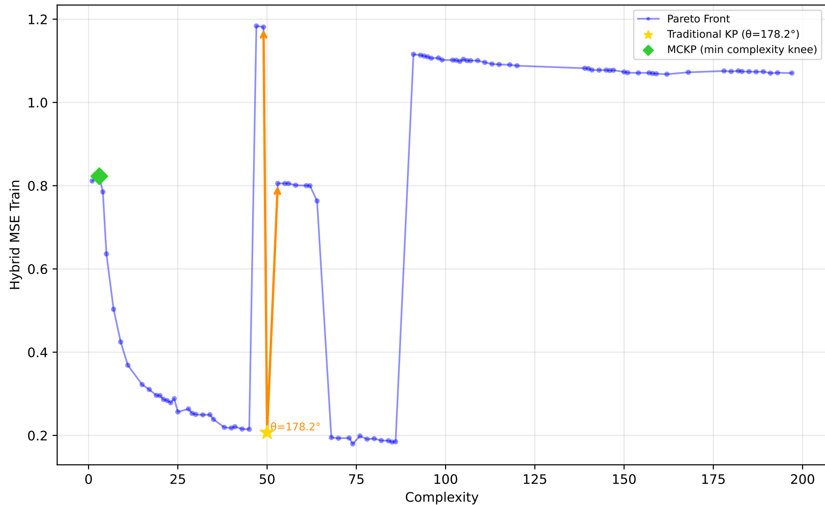
542_pollution - Run 19 - SVP - Hybrid MSE Train \lambda_1=0.70, \lambda_2=1.00, \lambda_3=0.10 | Difficulty: 0.72 | Method: hmr
